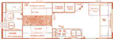
27' Rear Bath Travel Trailer Dry Weight - 4400 lbs. Hitch Weight - 500 lbs. Overall Length - 26' 11"
