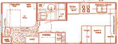
25' Center Bath Dinette Travel Trailer Dry Weight - 4000 lbs. Hitch Weight - 450 lbs. Overall Length - 24' 11"
