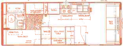
25' Rear Bath Bunks Travel Trailer Dry Weight - 4000 lbs. Hitch Weight - 450 lbs. Overall Length - 24' 11"
