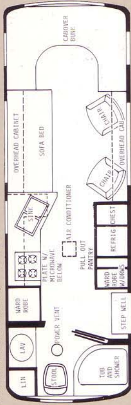
The 27' PRINCE 3 - Dry wt. 9600 lbs. - Overall length 26' 9"
