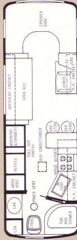
The 27' DUKE - Dry wt. 9600 lbs. - Overall length 26' 9"
