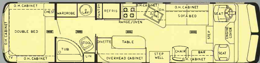
The 33' London Aire Class A - Dry Wt, 12,400 lbs. - Overall length 33'6" - Wheel base 220"
