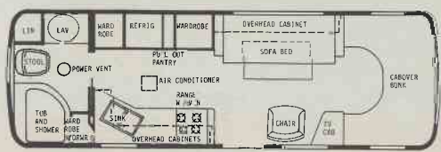
The 27' PRINCE 2 - Dry wt. 9,600 lbs. - Overall length 26' 9"
