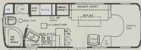
The 27' DUKE - Dry wt. 9,600 lbs. - Overall length 26' 9"
