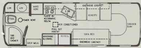
The 27' PRINCE I - Dry wt. 9,600 lbs. - Overall length 26' 9"
