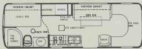
The 27' PRINCESS - Dry wt. 9,600 lbs. - Overall length 26' 9"
