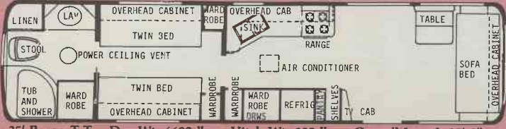
35' Baron T.T. - Dry Wt. 6600 lbs. - Hitch Wt. 900 lbs. - Overall Length 35' 8"
