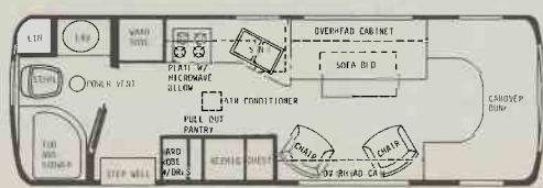
The 27' PRINCE 3 - Dry wt. 9,600 lbs. - Overall length 26' 9"
