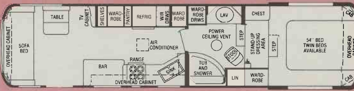
32' Statesman F.W. - Dry Wt. 7200 lbs. - Hitch Wt. 1750 lbs. - Overall Length 32' 9"
