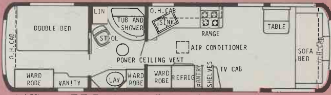
33' Viscount T.T. - Dry Wt. 6300 lbs. - Hitch Wt. 900 lbs. - Overall Length 33' 8"
