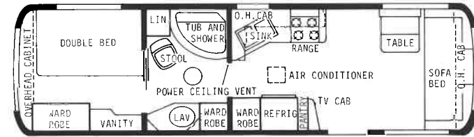
31' Viscount T.T. - Dry Wt. 6000 lbs. - Hitch Wt. 800 lbs. - Overall Length 31' 8"
