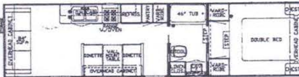
32' WALK THRU DINETTE
