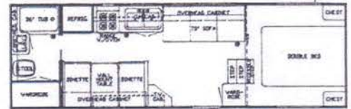
26' REAR BATH DINETTE
