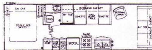
29' CENTER BATH DINETTE
