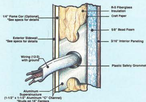
Sidewall Profile
