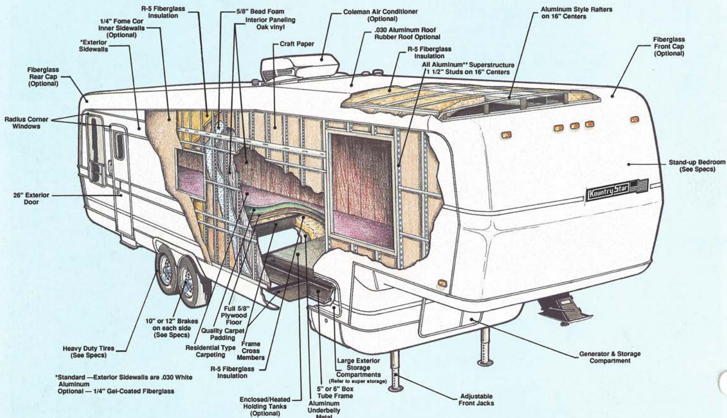
Sidewall Profile
