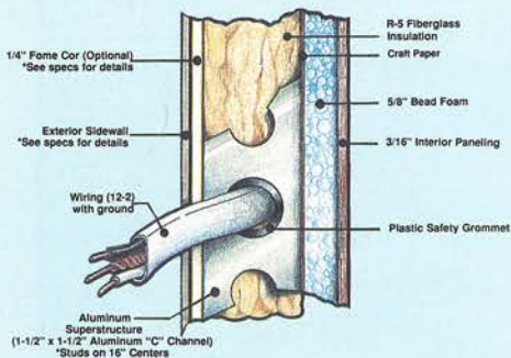
Sidewall Profile
