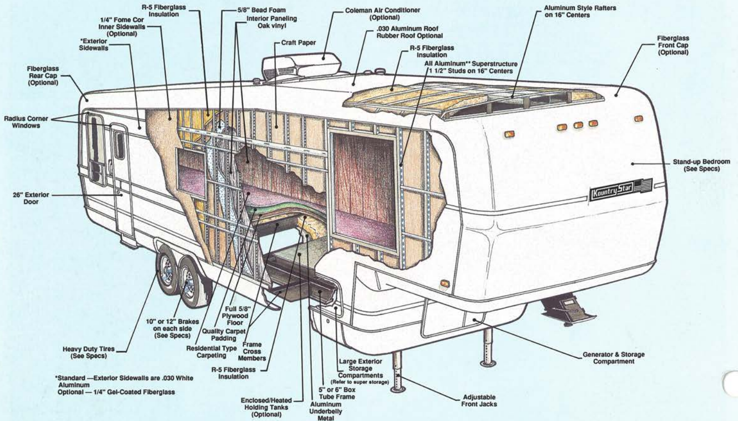
Sidewall Profile
