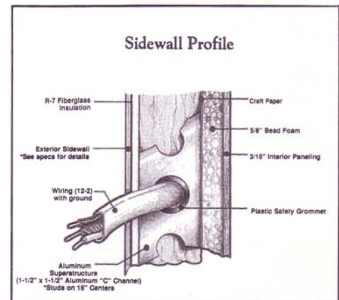
SIDEWALL PROFILE
