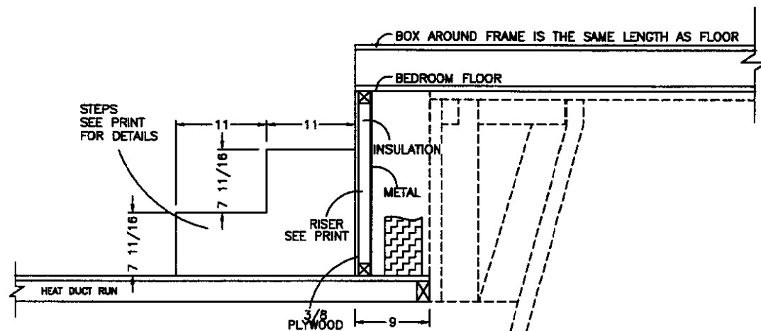
SIDE X-SECTION OF SUPER STORAGE
