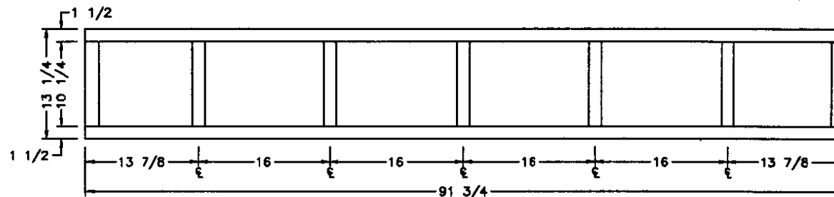
REAR SUPER STORAGE RISER RISER MADE UP w/2x2 STUDS. RISER SHOULD HAVE 3/16 PNLG ON BOTH SIDES
