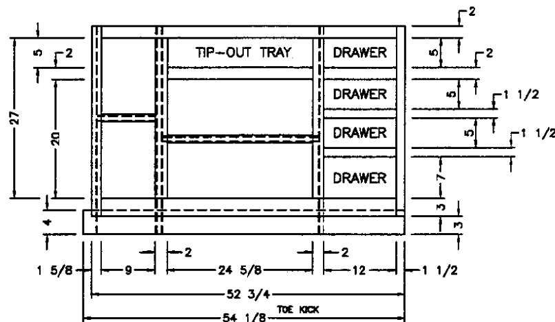
REAR KITCHEN BASE
