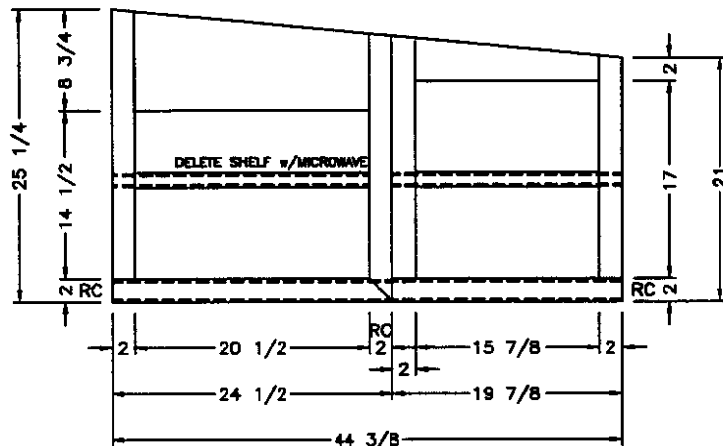
SIDE KITCHEN OVERHEAD 16 3/4" DEPTH 12" DEPTH
