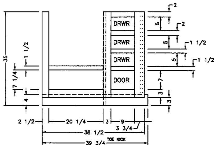
DOOR SIDE KITCHEN BASE
