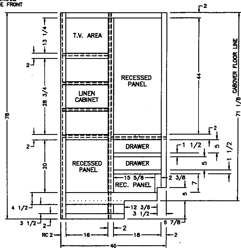
BEDROOM SIDE FRONT
