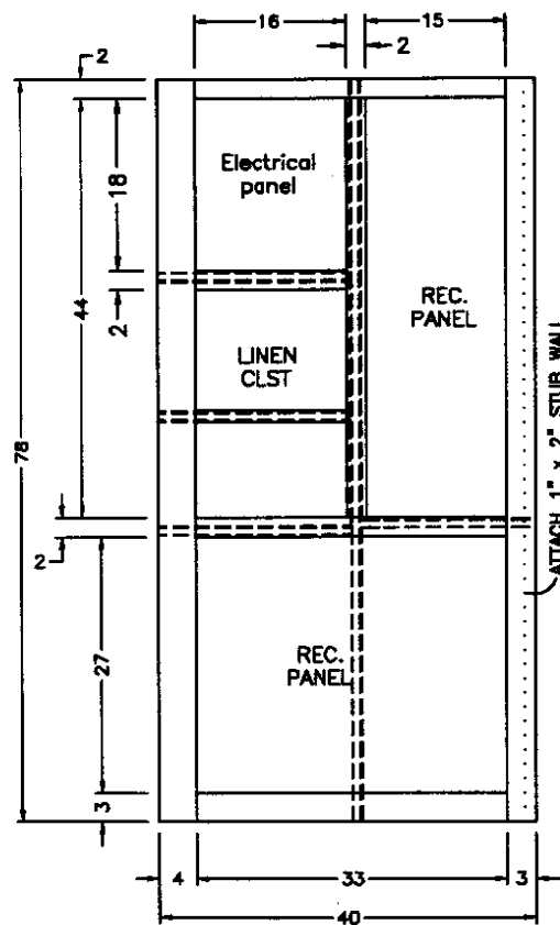
BATHROOM SIDE FRONT
