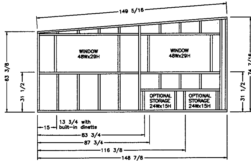
MAIN SLIDE-OUT SIDEWALL
