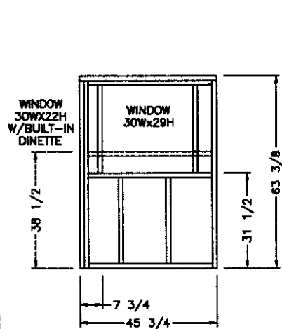
REAR SIDEWALL
