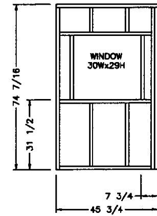
FRONT SIDEWALL
