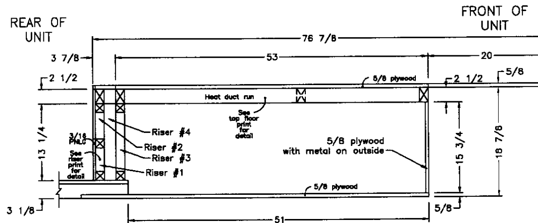
SIDE X-SECTION OF SUPER STORAGE BATHROOM FLOOR
