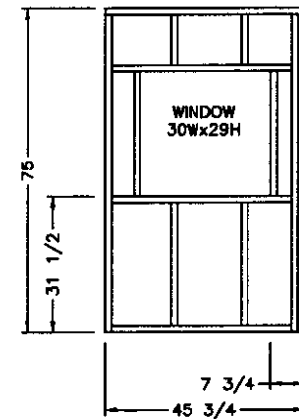
FRONT SIDEWALL
