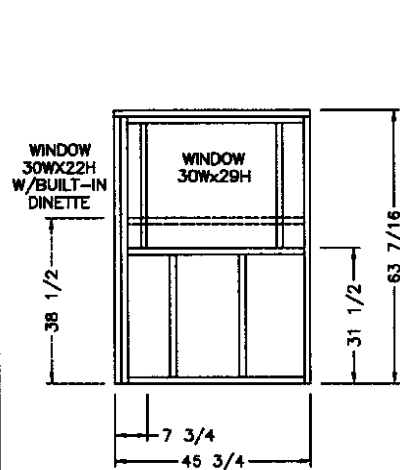
REAR SIDEWALL
