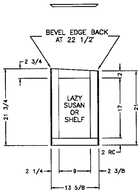
CORNER OVERHEAD (1) 9 1/2 X 17 1/2
