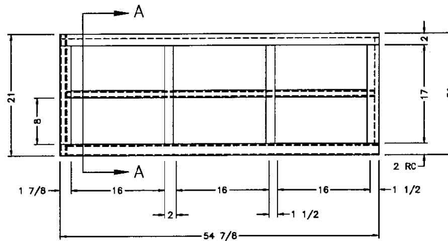
REAR OVERHEAD FRONT VIEW (3) 16 1/2 X 17 1/2 DOORS
