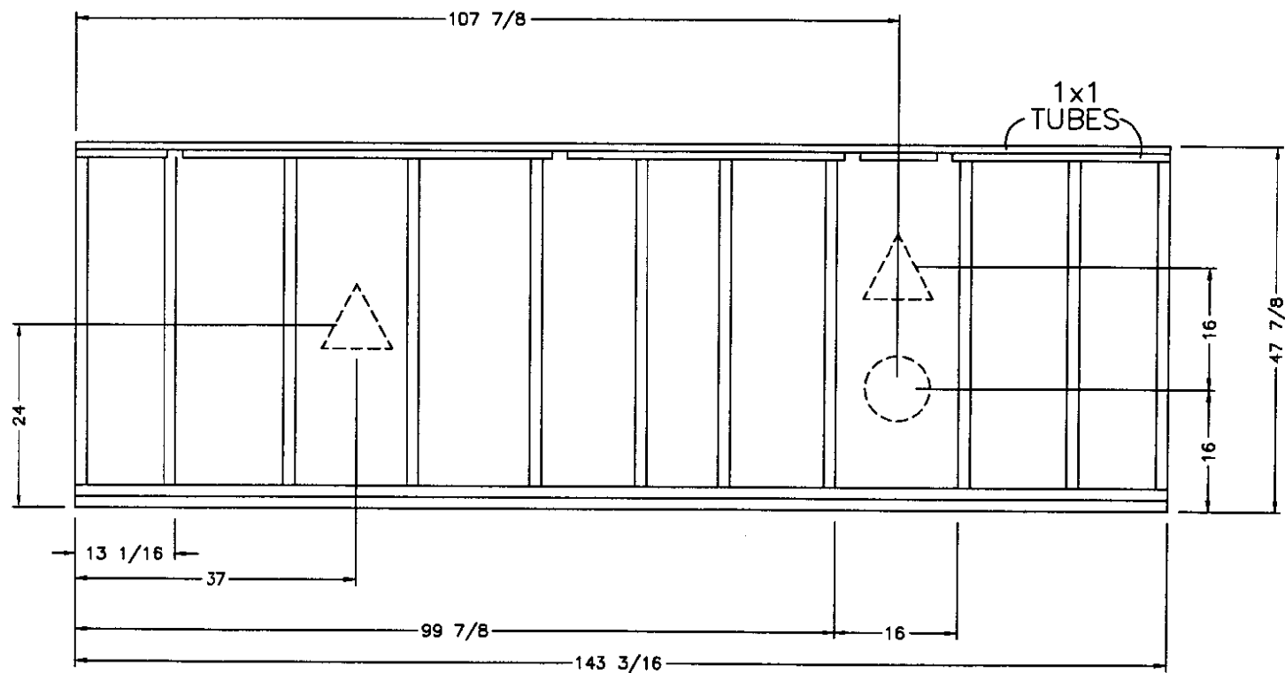
VIEW FROM OPEN SIDE LOOKING UP
