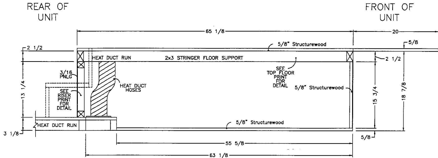
SIDE X-SECTION OF SUPER STORAGE BATHROOM
