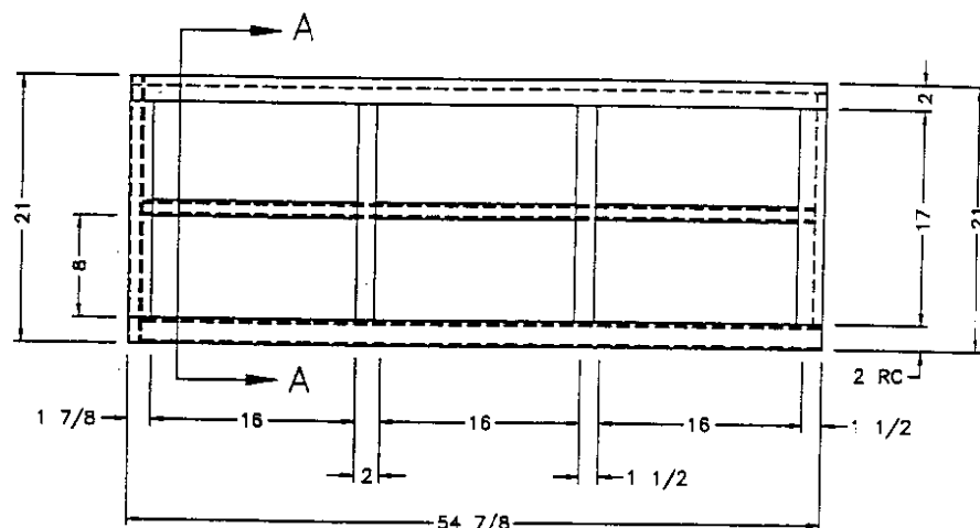
REAR OVERHEAD FRONT VIEW (3) 16 1/2 X 17 1/2 DOORS
