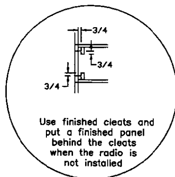
SECTION A-A RECESSED RADIO
