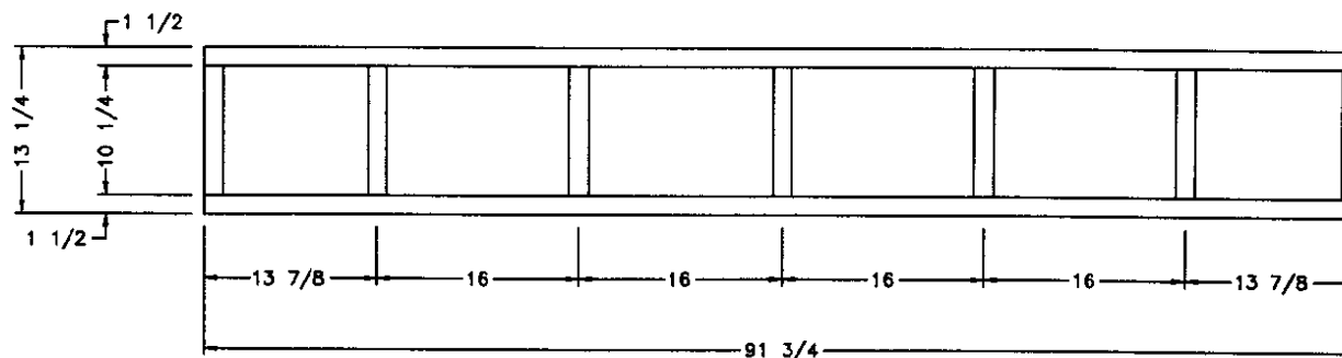
REAR SUPER STORAGE RISER RISER MADE UP w/2x2 STUDS. RISER SHOULD HAVE 3/16 PNLG ON BOTH SIDES
