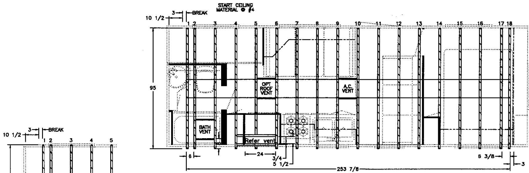
STANDARD ROOF LAYOUT
