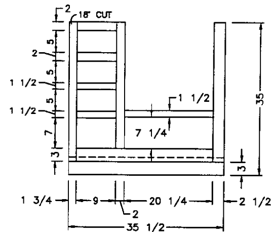
DRAWER/RANGE BASE
