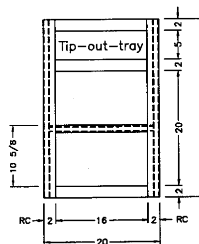
Lav Base 16" Deep (1) 16 1/2x20 1/2 Door (1) 16 1/2x5 3/4 Front
