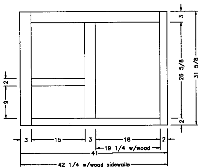
Ledge Base Framework Cover with Bathroom Wallboard
