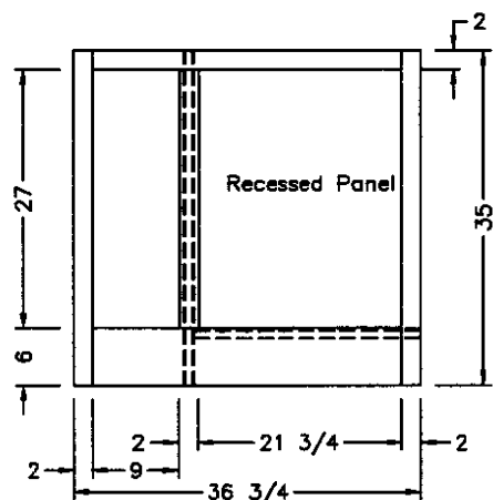
SIDE WING BASE (1) 9 1/2x27 1/2 Door
