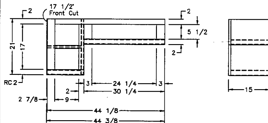
SPACEMAKER OVERHEAD (1) 24 1/2x6 1/2 Front (1) 9 1/2x17 1/2 Door
