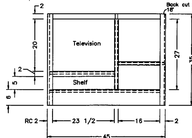
END WING BASE (1) 16 1/2x27 1/2 Door
