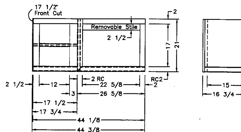
MICROWAVE OVERHEAD (2) 11 1/2x17 1/2 Doors (1) 12 1/2x17 1/2 Doors
