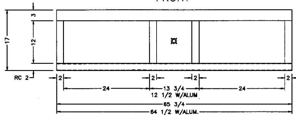
FRONT
