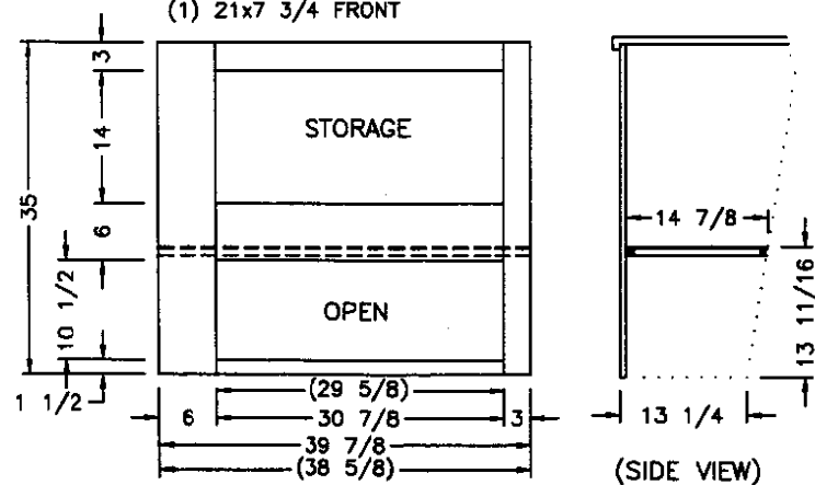
BUILT-IN DINETTE BASE
