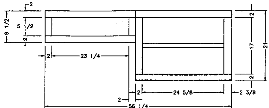
SIDE KITCHEN OVERHEAD W/SPACEMAKER
