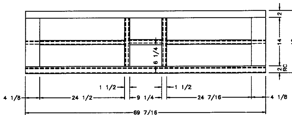
LIVINGROOM OVERHEAD FRONT VIEW
