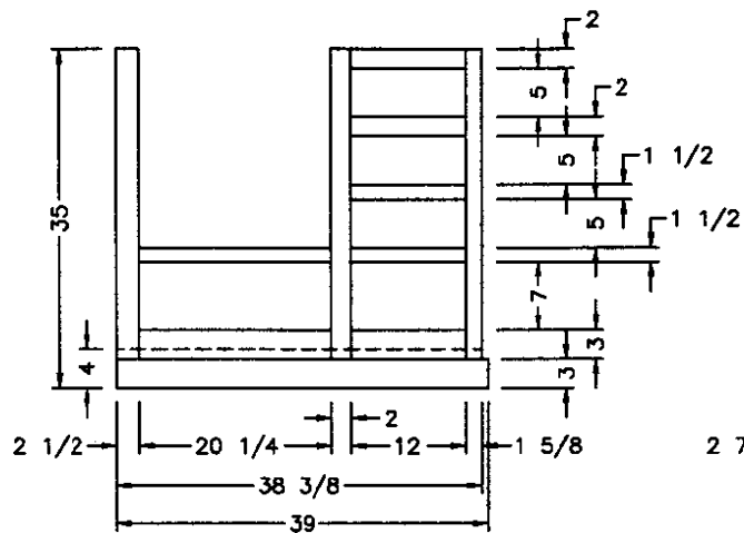
RANGE/DRAWER BASE
