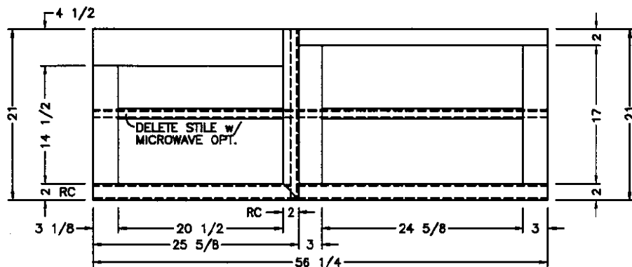
SIDE KITCHEN OVERHEAD W/MICROWAVE
