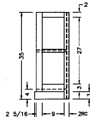
REAR WING BASE
