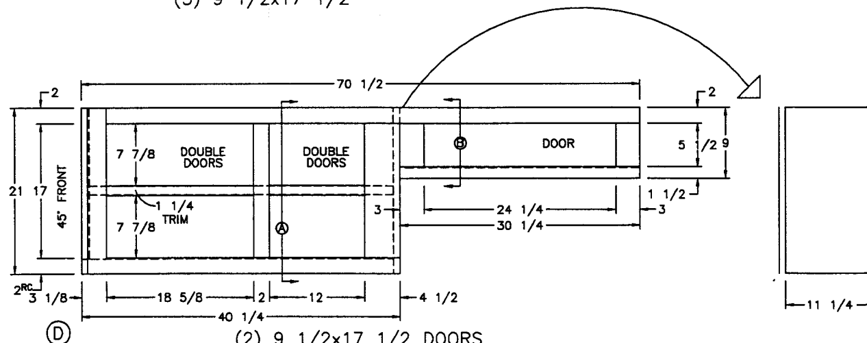
(2) 9 1/2x17 1/2 DOORS (1) 12 1/2x17 1/2 DOOR (1) 24 3/4x6 DOOR
