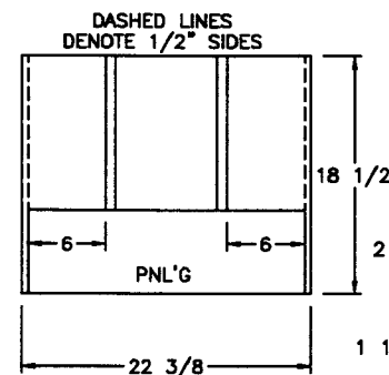
DETAIL C - BOTTOM 1/2" PLYW'D
