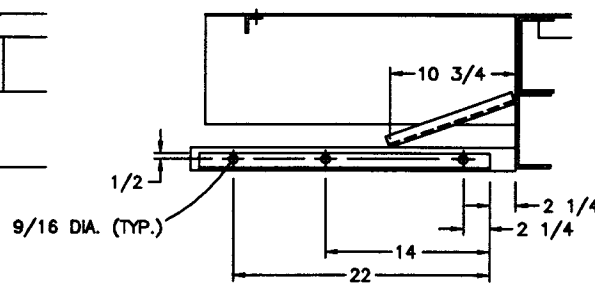
REAR-FACING SIDE VIEW
