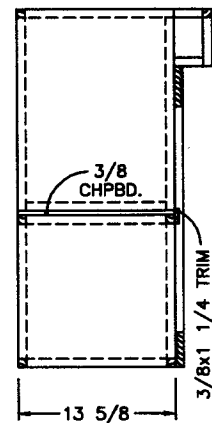
SIDE SECTION (A)
