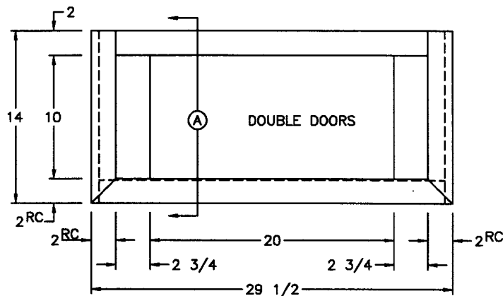
FRONT VIEW (1) 20 1/2x10 1/2 DOOR
