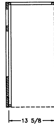
SIDE SECTION (B)
