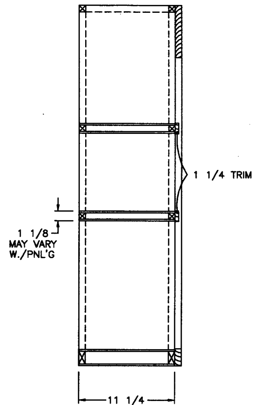
SIDE SECTION (A)
