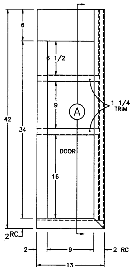
FRONT VIEW
