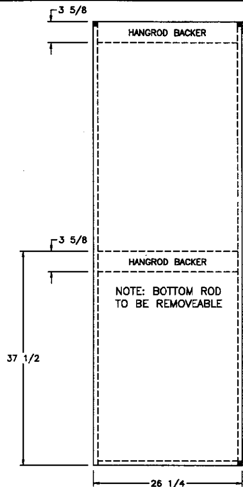
SIDE SECTION (A) (2) 12 1/2x71 1/2 MIRROR DOORS
