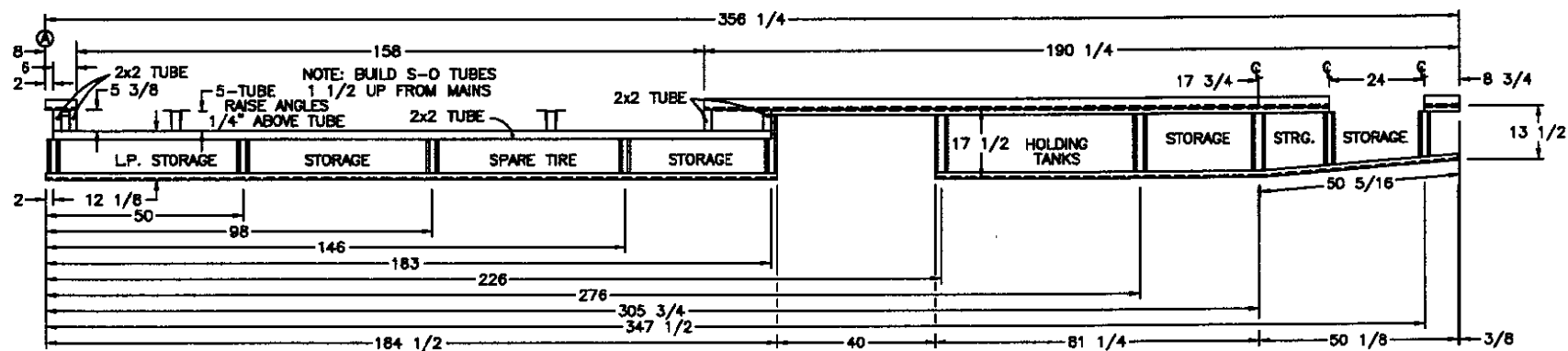
OFFDOOR SIDE
