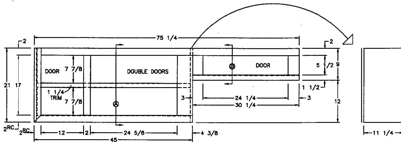
FRONT VIEW
