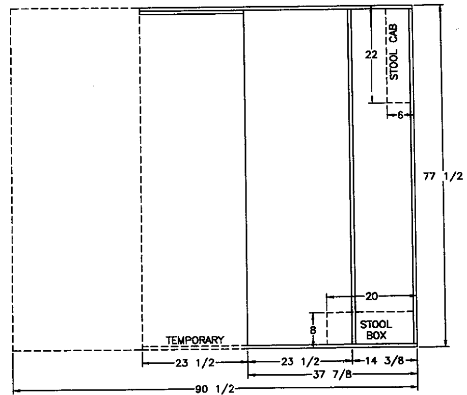
VIEW (B)
