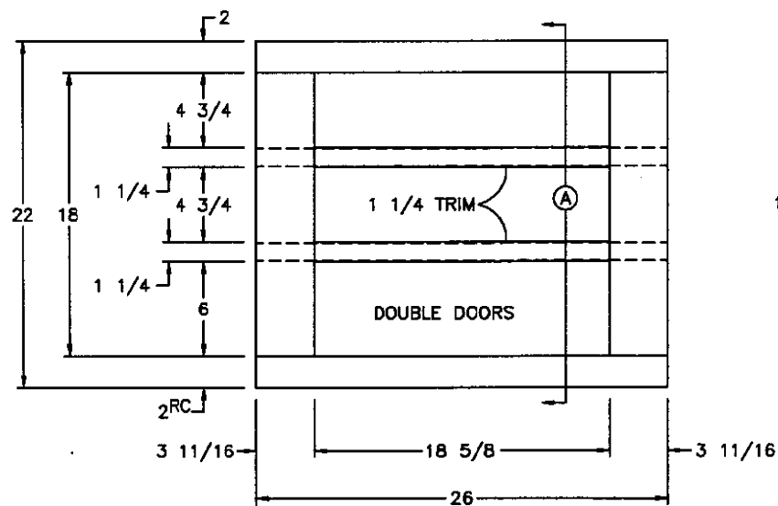
FRONT VIEW (2) 9 1/2x18 1/2 DOORS
