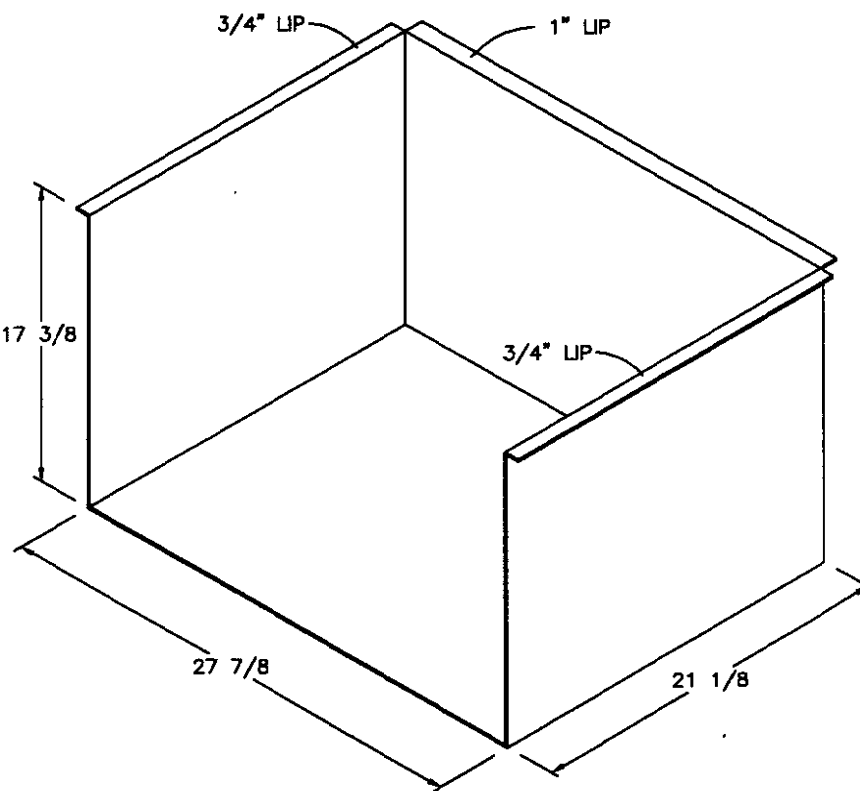
OFFDOOR SIDE
