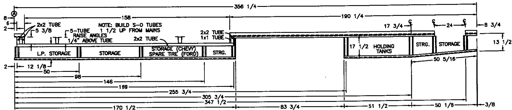
OFFDOOR SIDE
