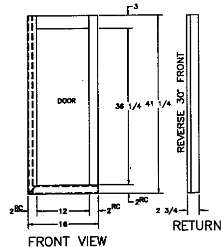
OFFDOOR SIDE
