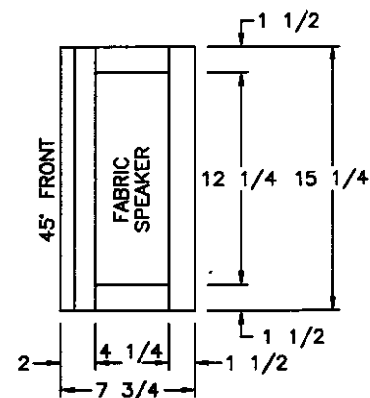
RT END VIEW
