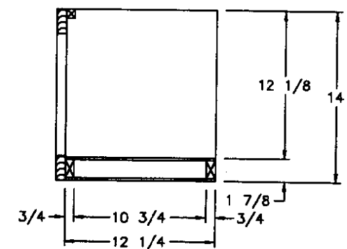
SIDE SECTION (A)
