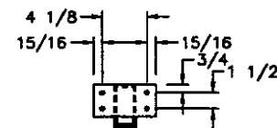
END VIEW
