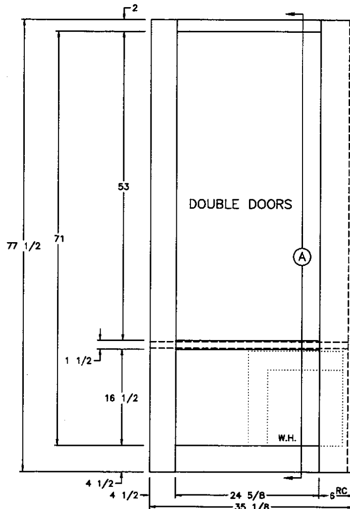
FRONT VIEW
