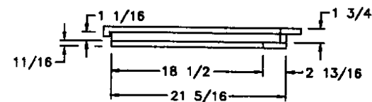
SIDE SECTION
