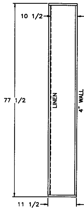
VIEW (E)
