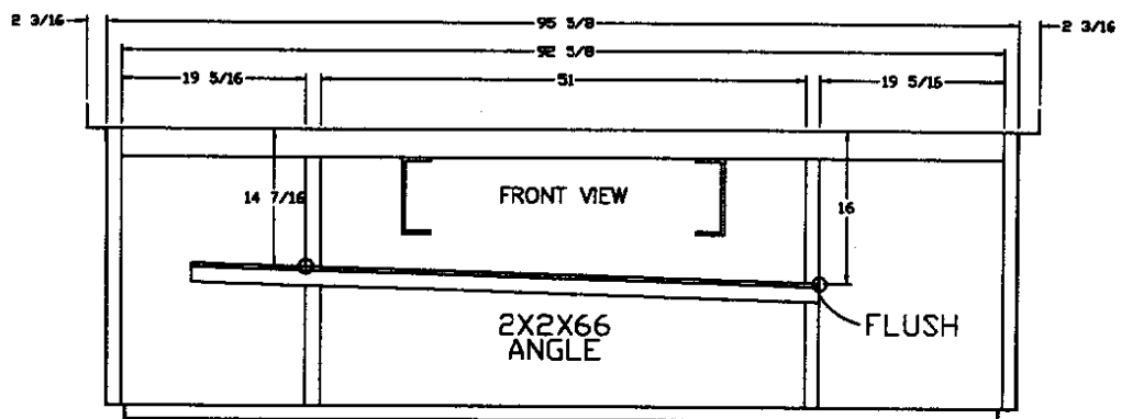
REAR HOLDING TANK CROSSMEMBER
