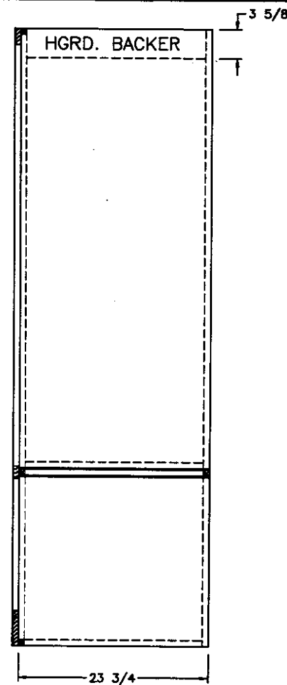
SIDE SECTION (A) (2) 12 1/2x71 1/2 MIRROR DOORS
