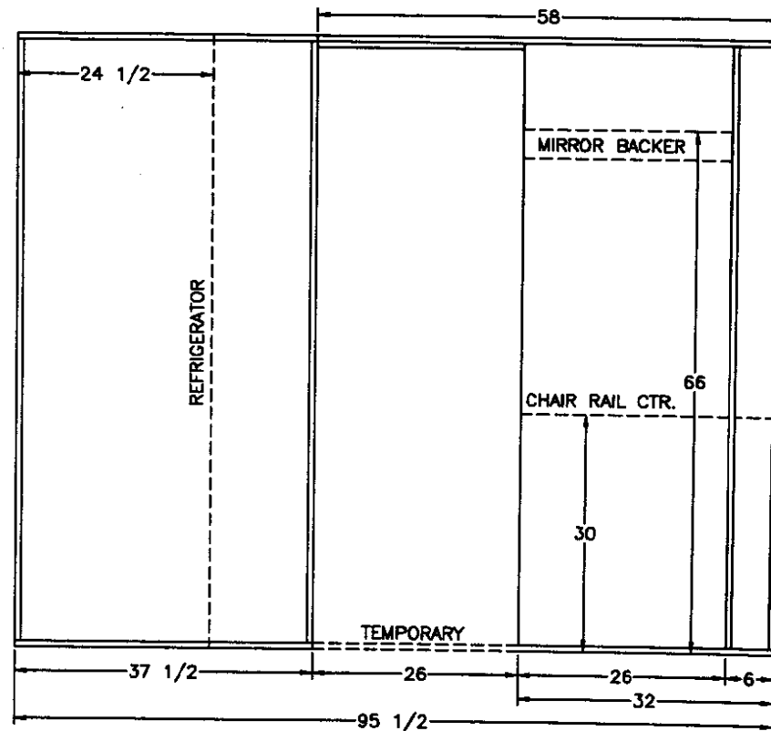
VIEW D
