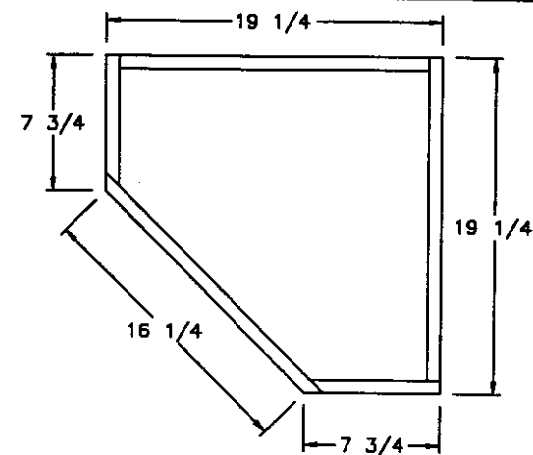
BOTTOM PANEL
