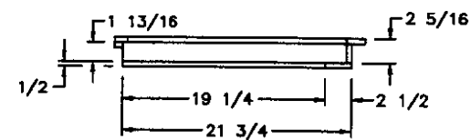
SIDE SECTION
