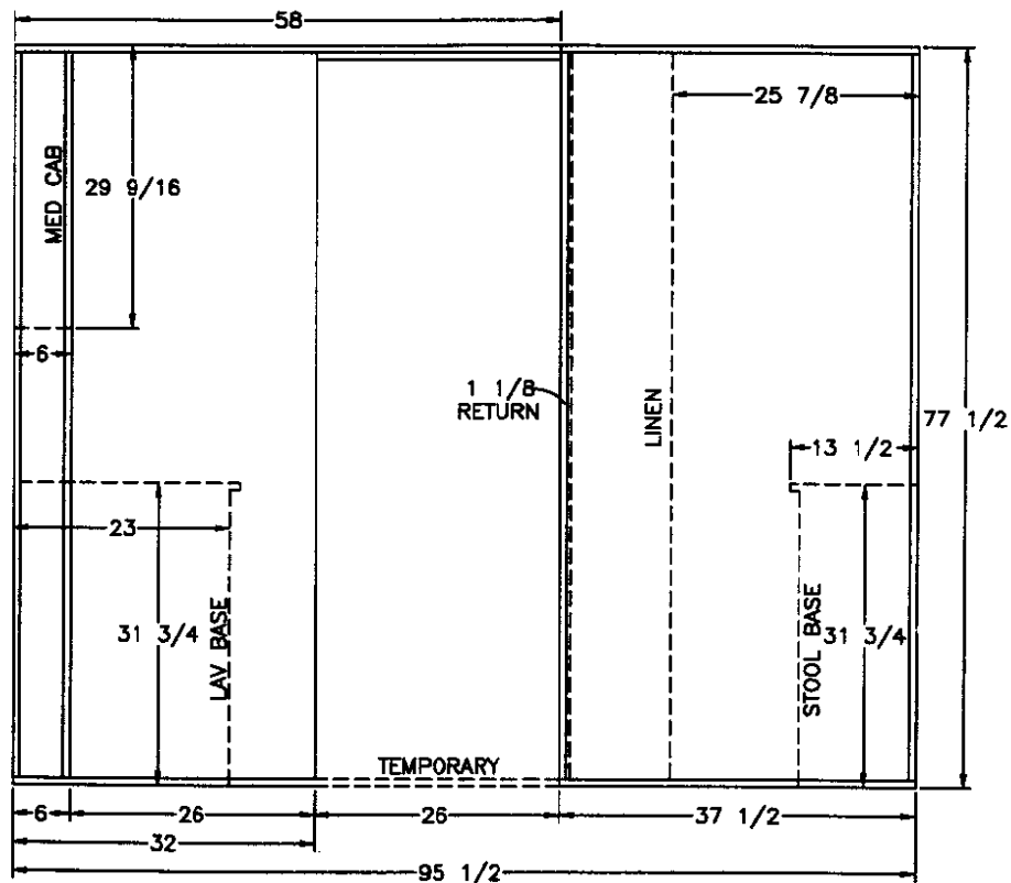
VIEW C
