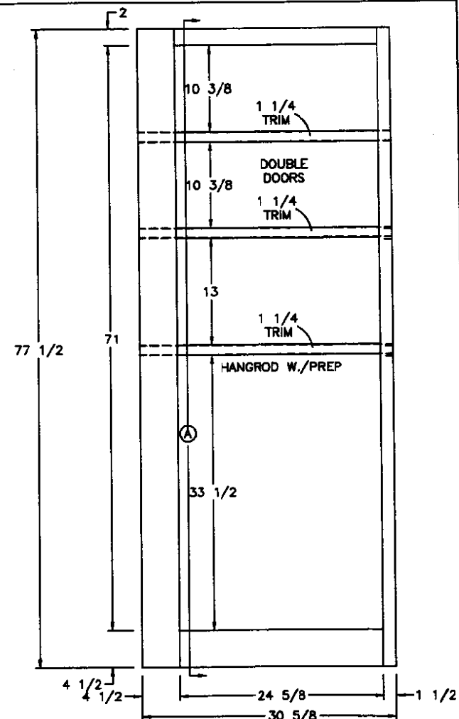
FRONT VIEW
