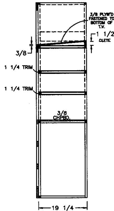
SIDE SECTION (B)
