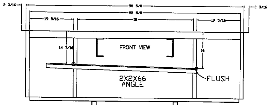
REAR HOLDING TANK CROSSMEMBER
