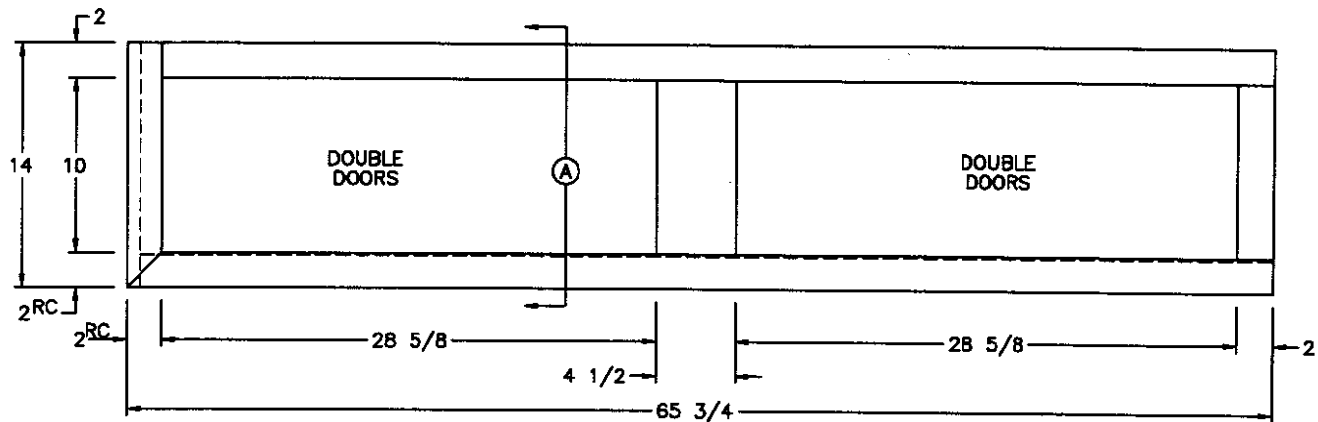
FRONT VIEW (4) 14 1/2x10 1/2 DOORS
