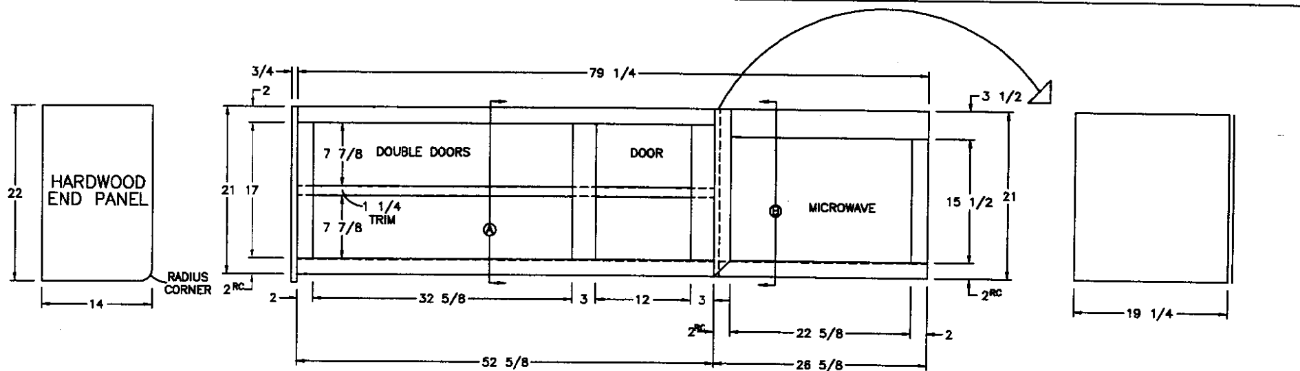
FRONT VIEW
