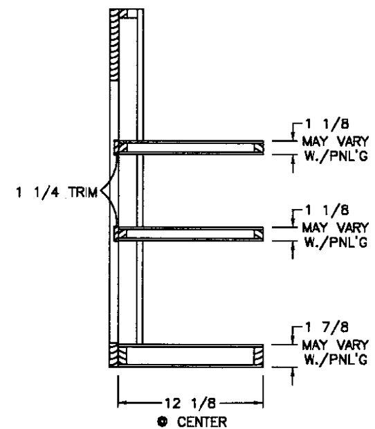
SIDE SECTION (A)
