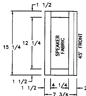
LFT END VIEW
