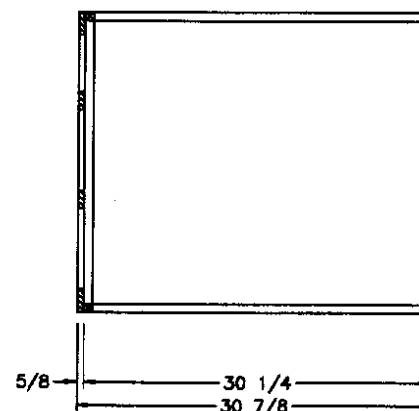
SIDE SECTION (B)
