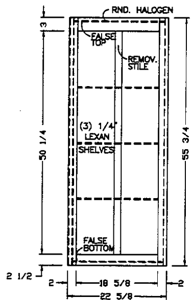
CHINA HUTCH OVERHEAD FRONT VIEW
