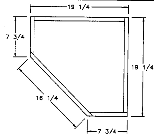
BOTTOM PANEL
