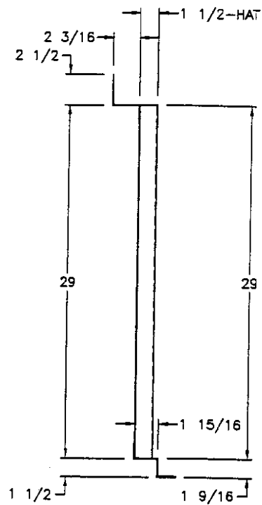
SIDE PROFILE (A)
