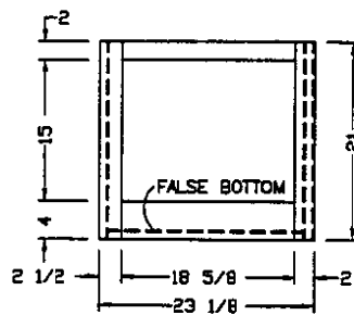
CHINA HUTCH BASE FRONT VIEW
