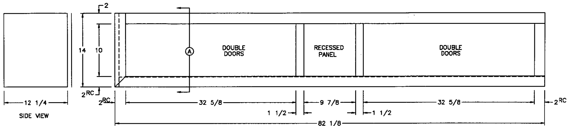
FRONT VIEW (4) 16 1/2x10 1/2 DOORS
