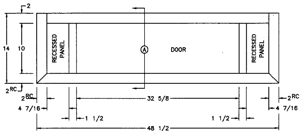
FRONT VIEW (2) 16 1/2x10 1/2 GLASS DOORS
