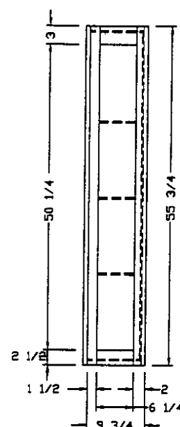
CHINA HUTCH OVERHEAD SIDE VIEW
