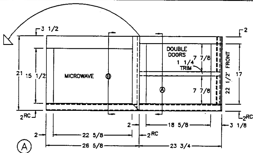
(2) 9 1/2x17 1/2 DOORS
