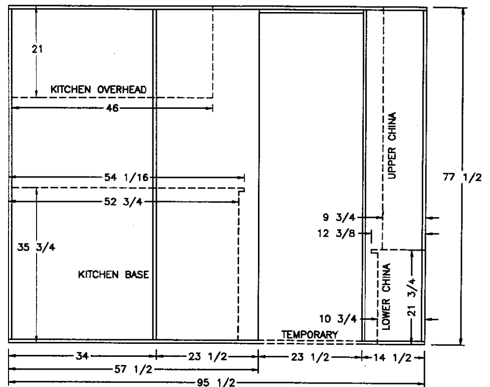
VIEW D
