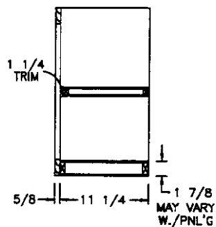
SIDE SECTION A
