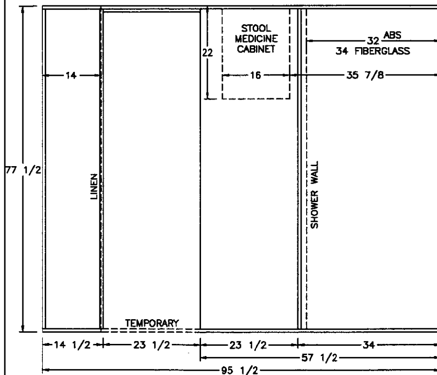
VIEW C
