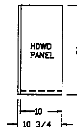
MP 4058/ LP 4057 CHINA HUTCH BASE SIDE VIEW
