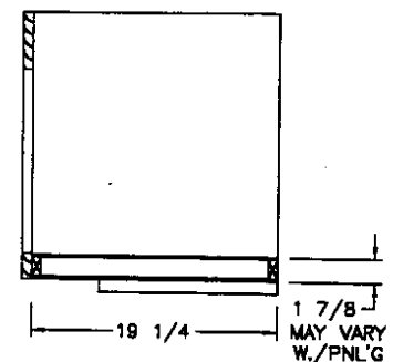
SIDE SECTION (B)
