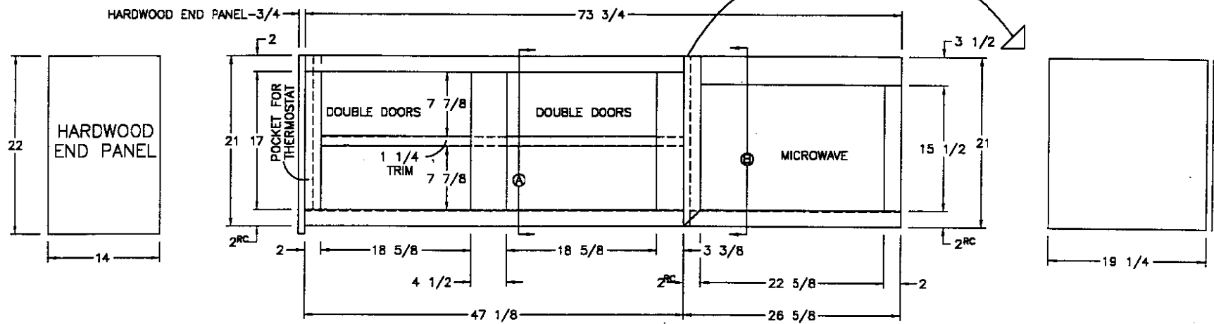
FRONT VIEW (4) 9 1/2x17 1/2 DOORS
