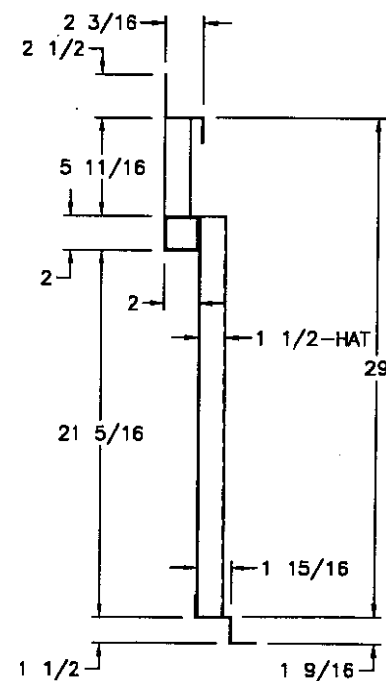
SIDE PROFILE (B)
