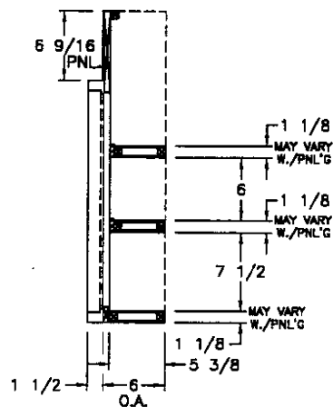
SIDE SECTION A-A
