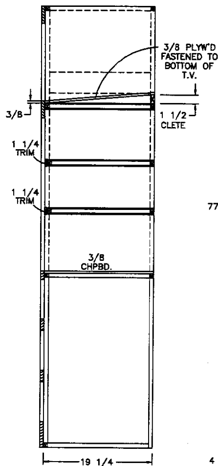
SIDE SECTION B
