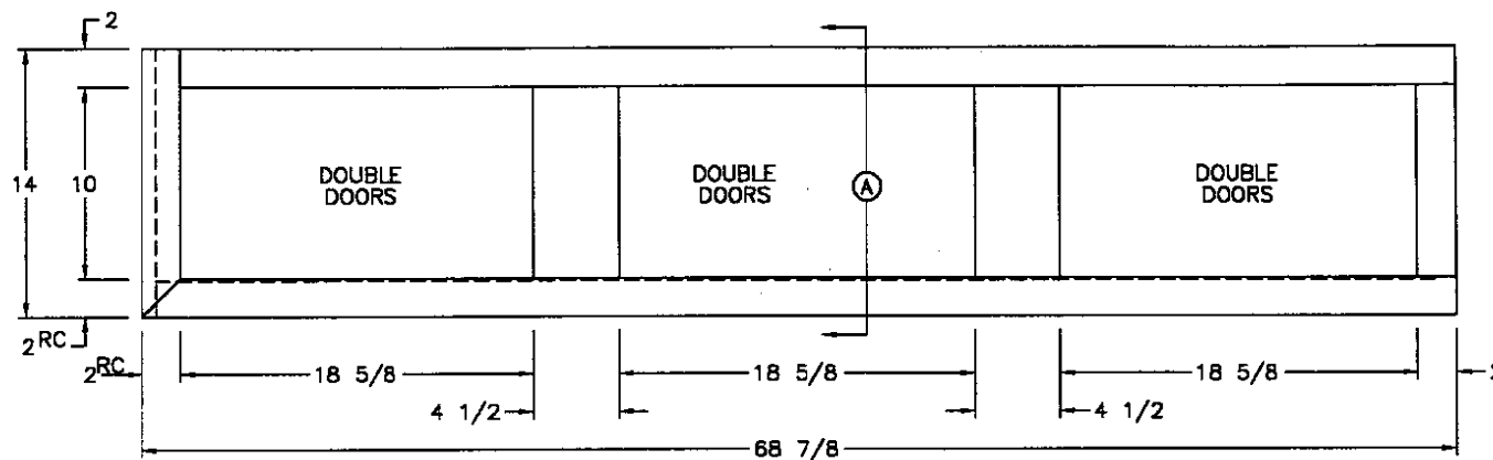
FRONT VIEW (6) 9 1/2 x 10 1/2 DOORS
