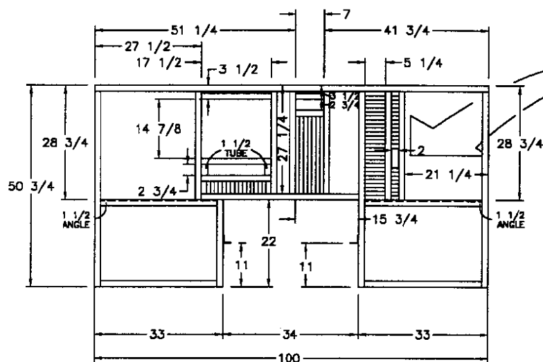
1 1/2 TUBES FRONT/EXTERIOR VIEW
