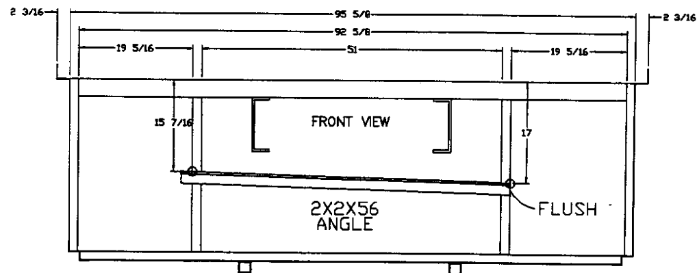
REAR HOLDING TANK CROSSMEMBER
