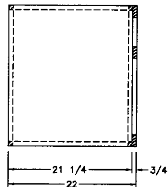
SIDE SECTION (A)
