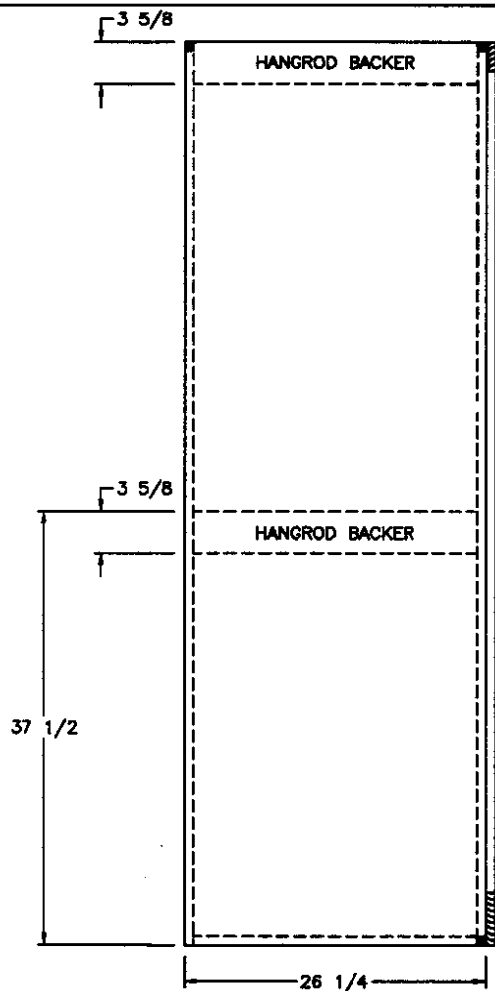
SIDE SECTION (A) (2) 12 1/2x71 1/2 MIRROR DOORS
