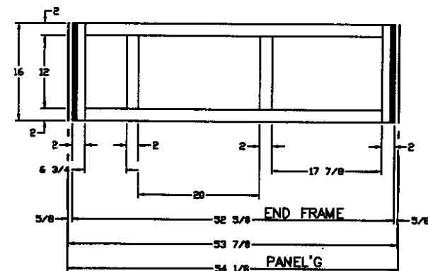
END (INTERIOR VIEW)
