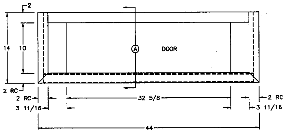
FRONT VIEW (2) 16 1/2x10 1/2 GLASS DOORS
