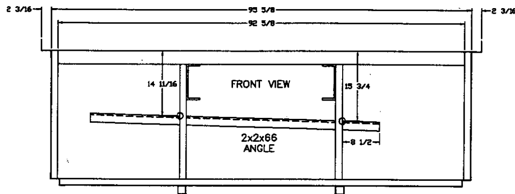
FRONT HOLDING TANK CROSSMEMBER
