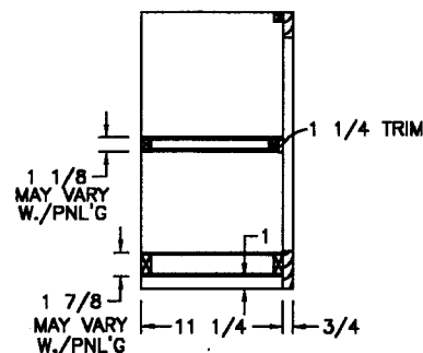
SIDE SECTION (A)
