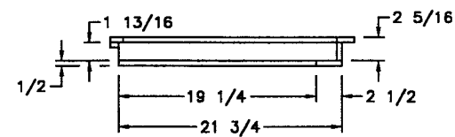
SIDE SECTION
