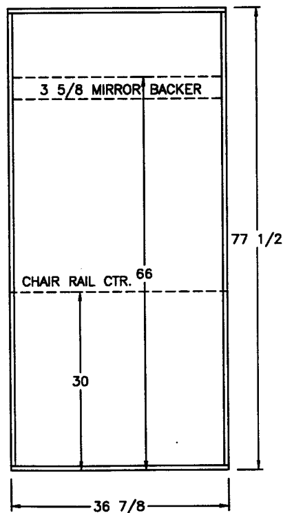
VIEW (C)
