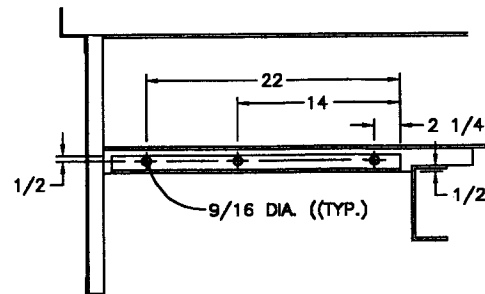
REAR-FACING SIDE VIEW
