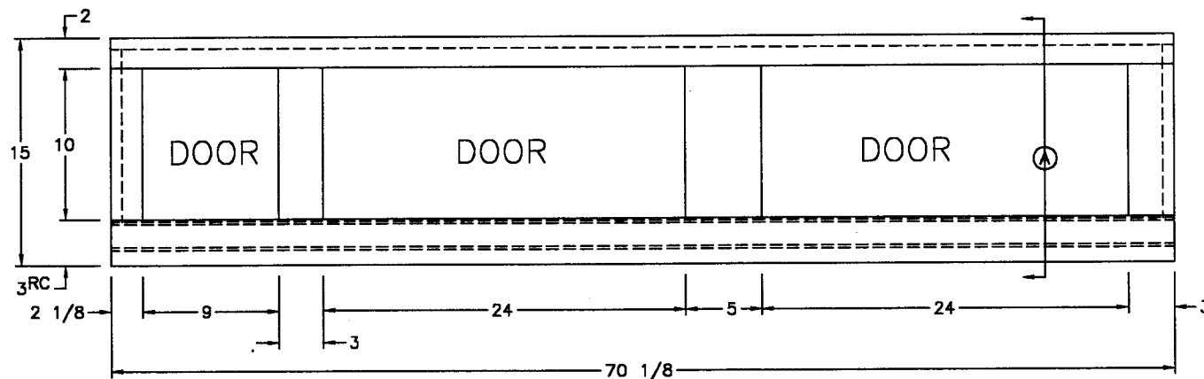
FRONT VIEW
