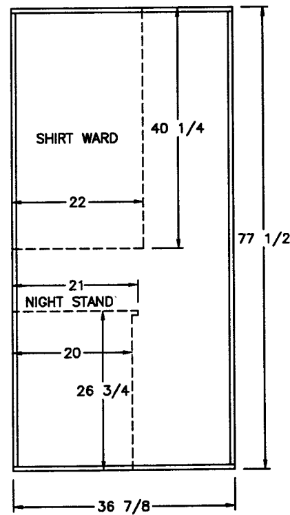
VIEW (E)
