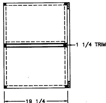
SIDE SECTION (A)
