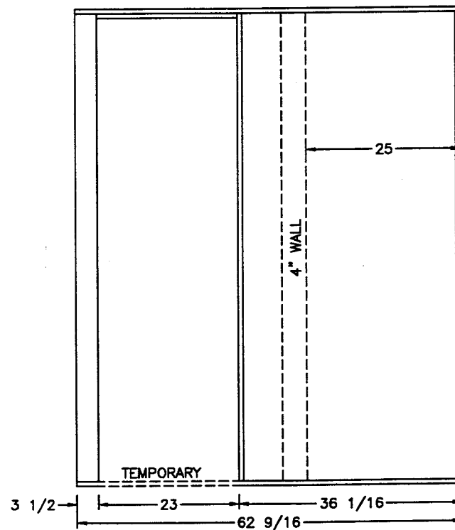
VIEW (H)
