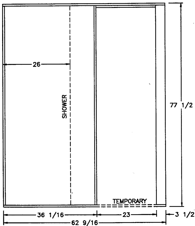
VIEW (G)
