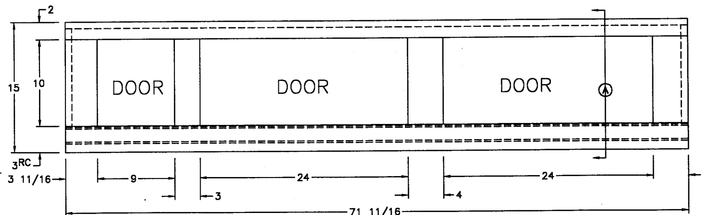
FRONT VIEW
