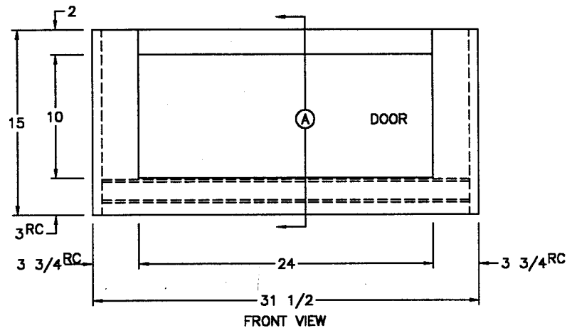
(1) 24 1/2x11 1/2 GLASS DOOR
