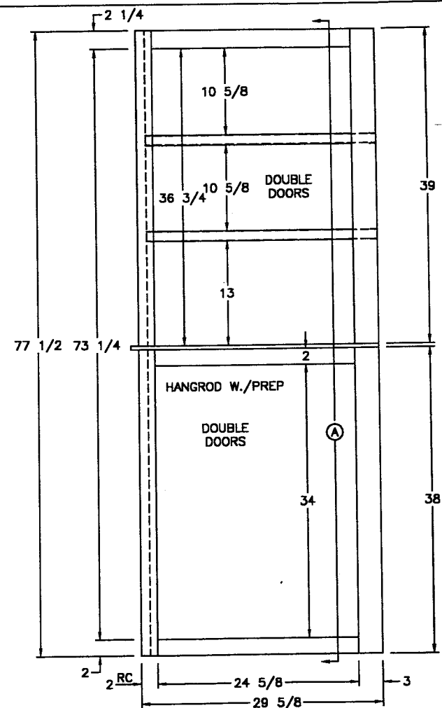
FRONT VIEW
