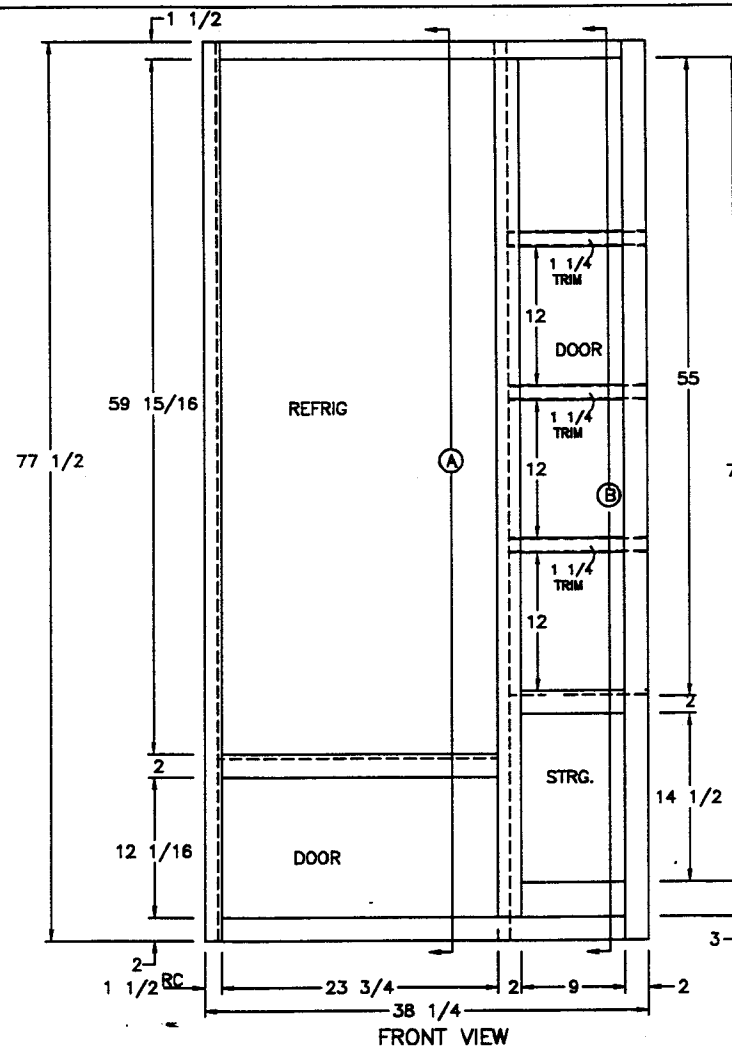
FRONT VIEW
