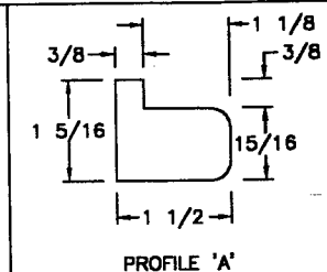
PROFILE 'A'
