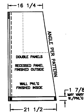
SIDE SECTION ©
