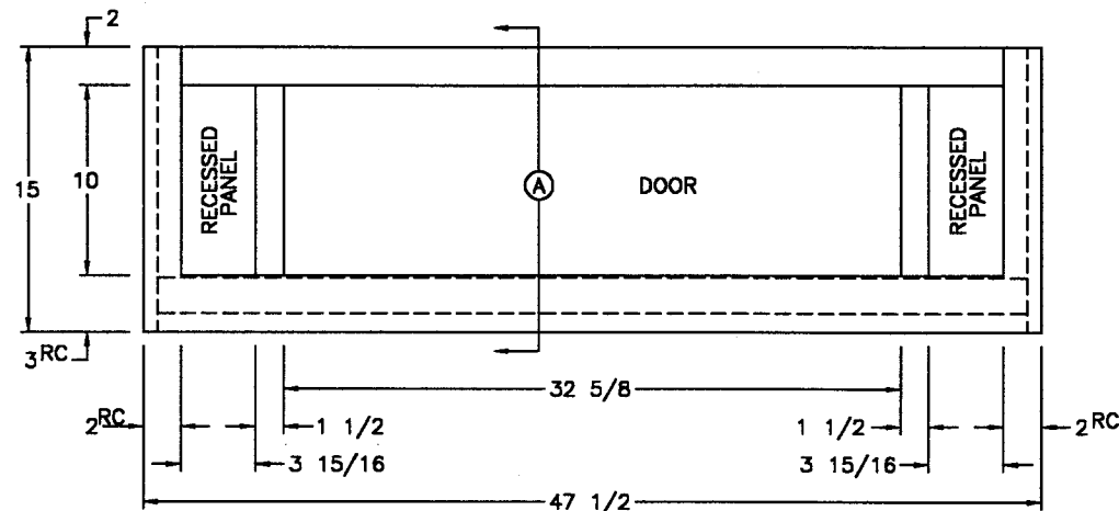
FRONT VIEW (2) 16 1/2x11 1/2 GLASS DOORS
