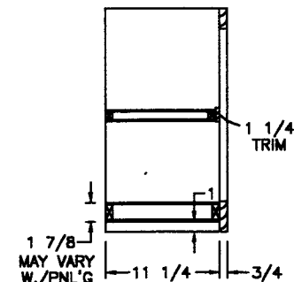
SIDE SECTION C
