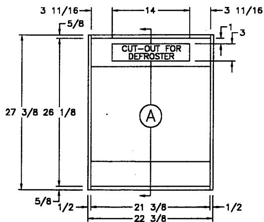
FRONT VIEW (FRAME)
