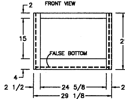
CHINA HUTCH BASE FRONT VIEW
