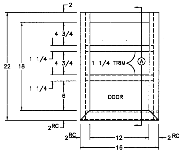
FRONT VIEW (1) 12 1/2x18 1/2 DOOR
