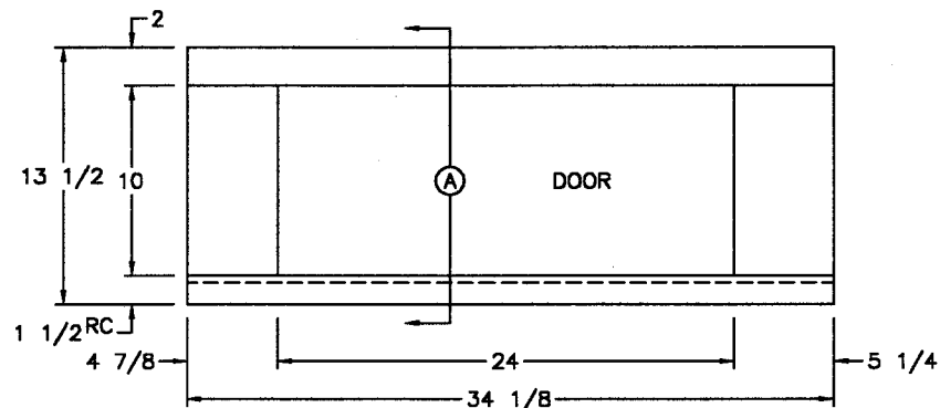
FRONT VIEW (1) 24 1/2x10 1/2 DOOR
