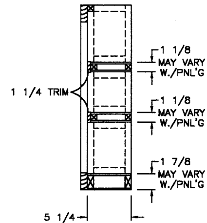
SIDE SECTION (A)
