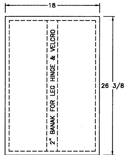
DOTTED LINES DENOTE BUILD-UP TOP VIEW OF TABLE
