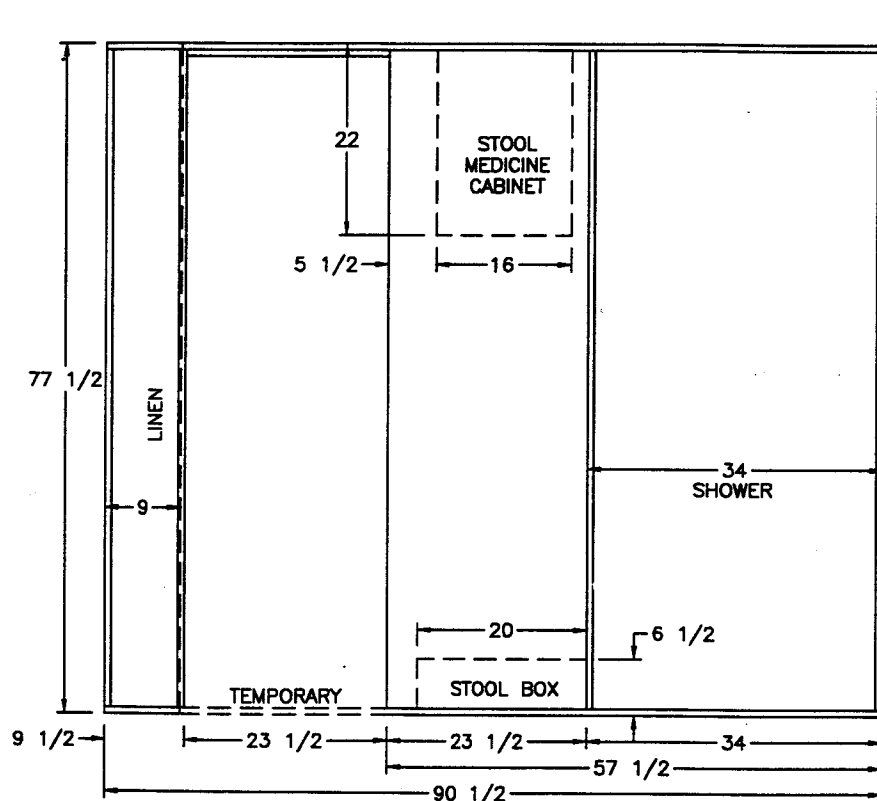
VIEW C
