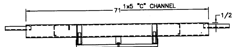
REAR END VIEW
