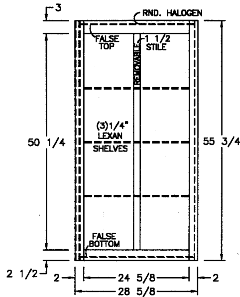
CHINA HUTCH OVERHEAD FRONT VIEW
