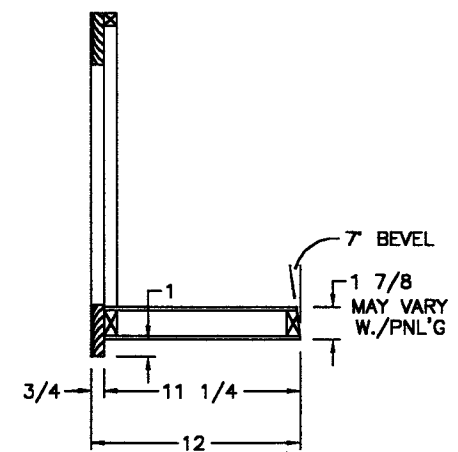
SIDE SECTION (A)
