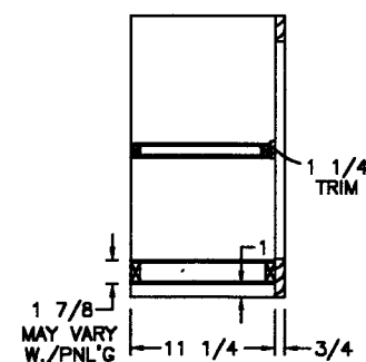
SIDE SECTION (C)
