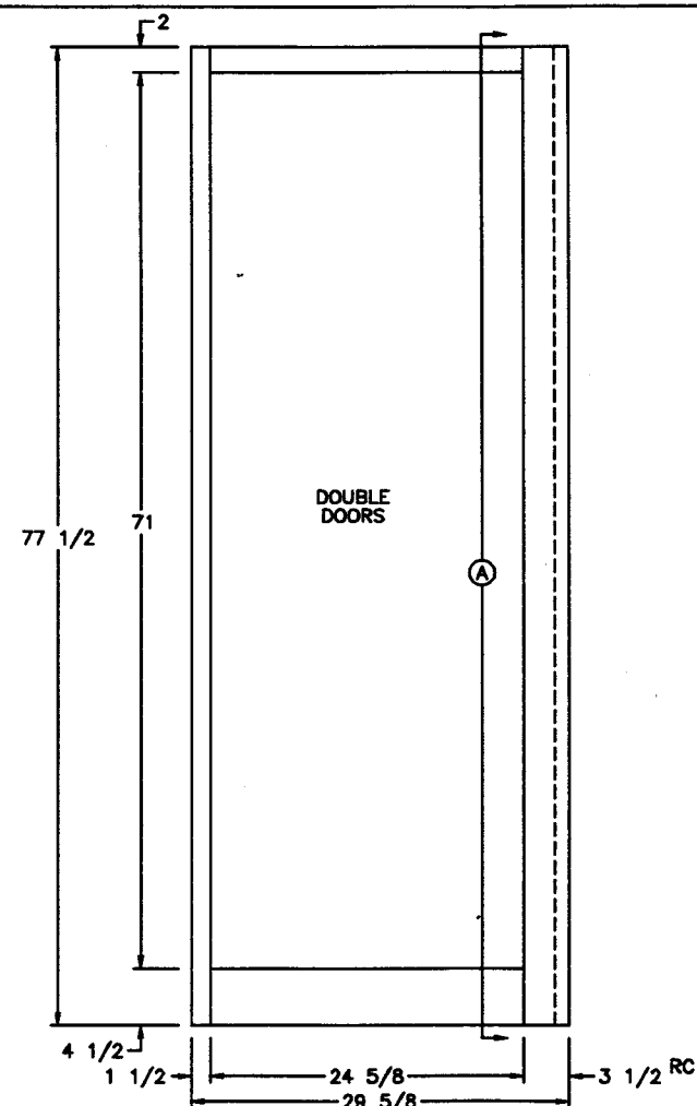
FRONT VIEW
