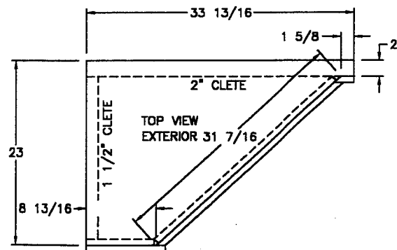
OFFDOOR SIDE
