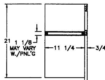
SIDE SECTION (B)
