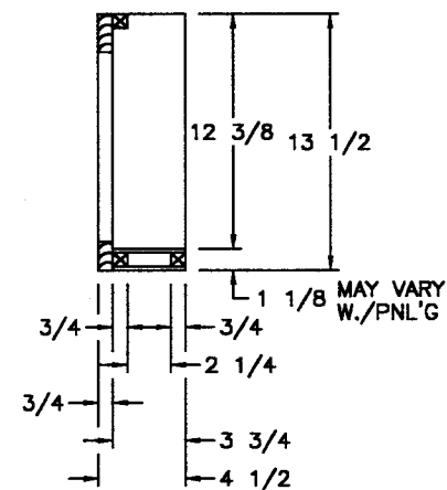
SIDE SECTION (A)
