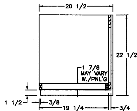
SIDE SECTION B
