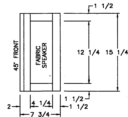
RT END VIEW
