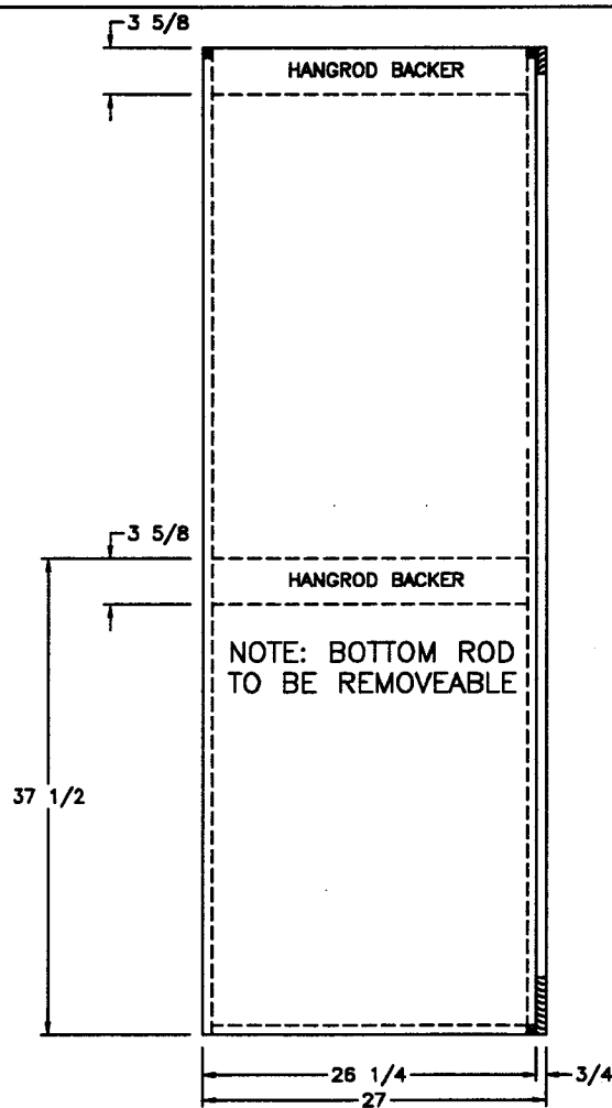
SIDE SECTION (A) (2) 12 1/2x71 1/2 MIRROR DOORS
