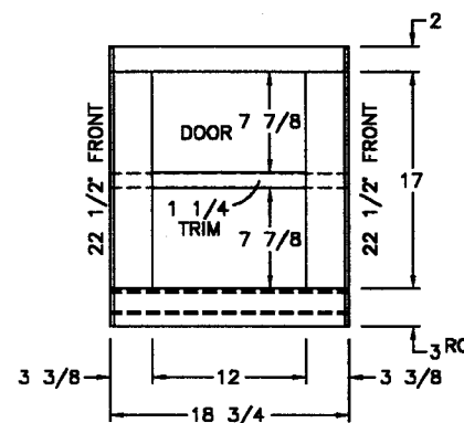
(1) 12 1/2x18 1/2 DOORS
