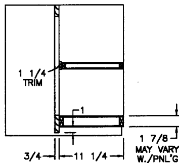
SIDE SECTION A
