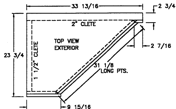
OFFDOOR SIDE
