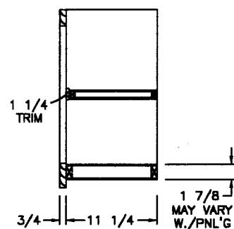
SIDE SECTION (A)
