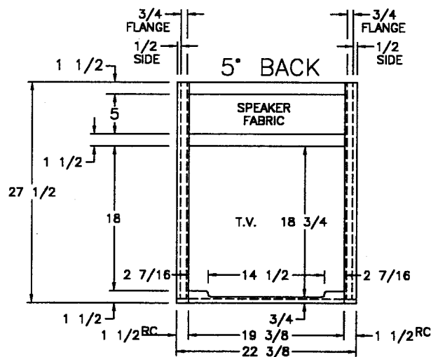
FRONT VIEW (FRONT)
