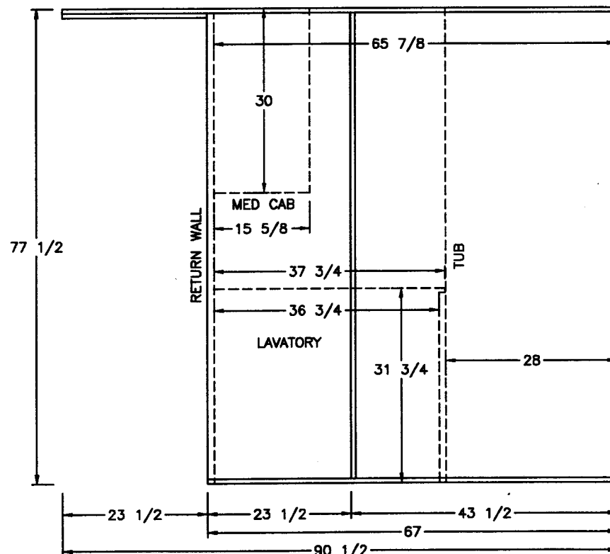
VIEW (B)
