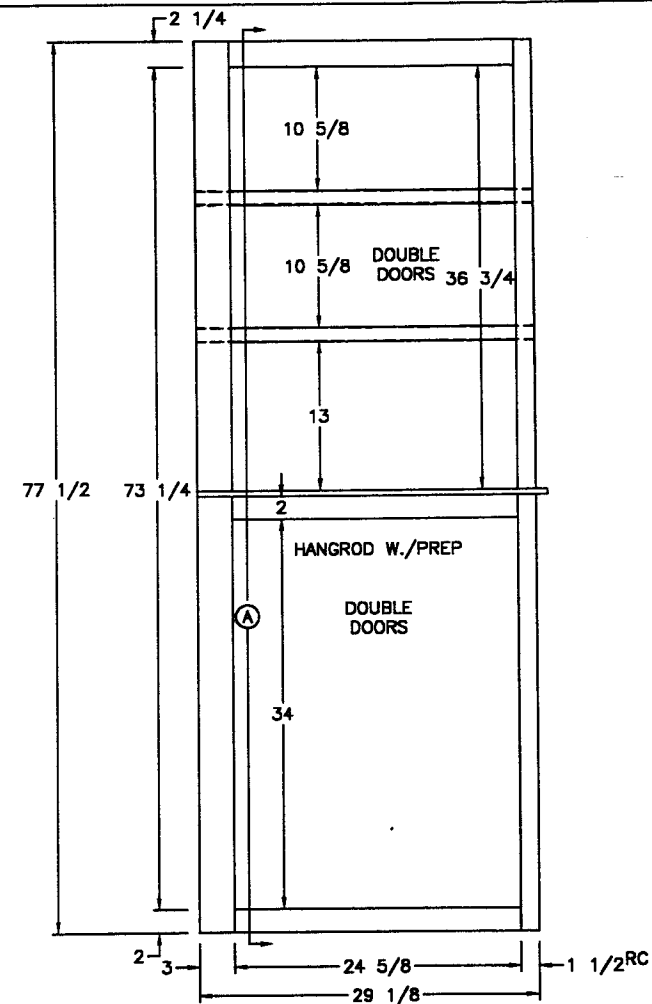
FRONT VIEW
