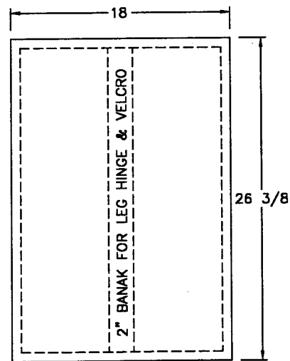
TOP VIEW OF TABLE
