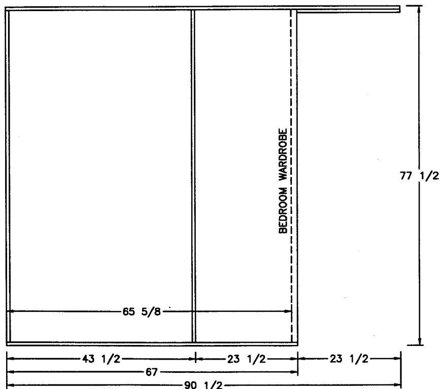
VIEW (A)
