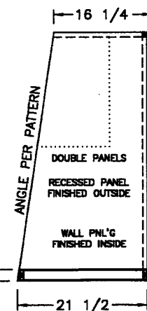
SIDE SECTION (C)
