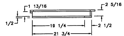
SIDE SECTION
