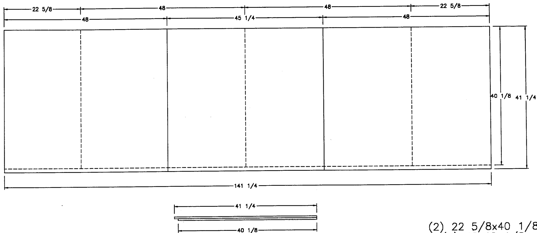
FRONT END VIEW
