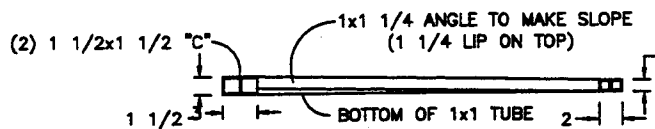
END VIEW—RIGHT SIDE UP
