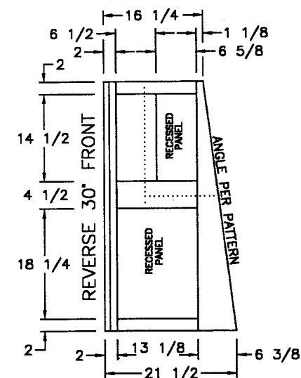
END PANEL
