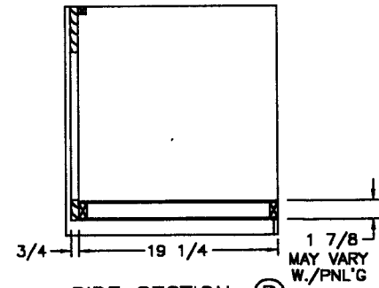
SIDE SECTION (B)
