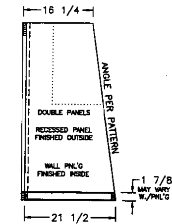
SIDE SECTION ©
