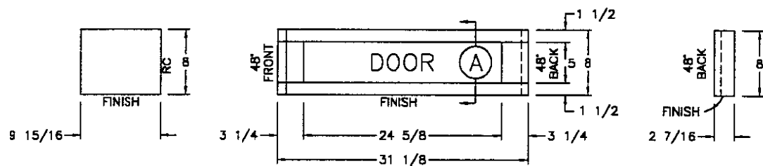
OFFDOOR SIDE FRONTS (1) 25 1/8x5 1/2 DOOR
