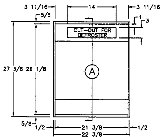
FRONT VIEW (FRAME)
