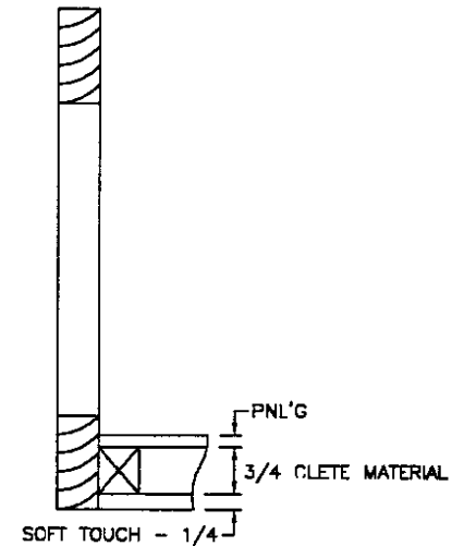
SIDE SECTION (A) ENLARGED 5X
