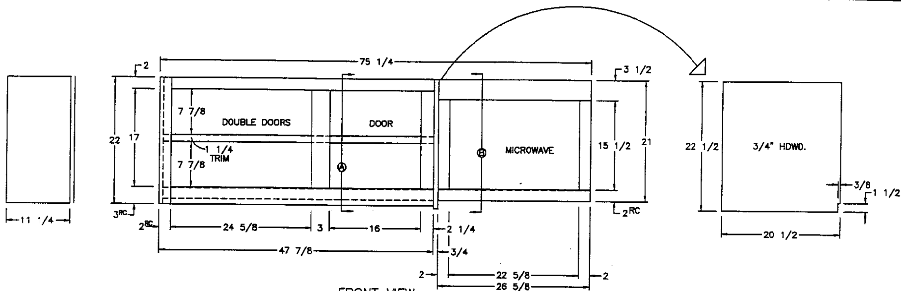
FRONT VIEW (2) 12 \frac{1}{2} x 18 \frac{1}{2} DOORS (1) 16 \frac{1}{2} x 18 \frac{1}{2} DOORS
