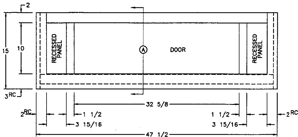
FRONT VIEW
