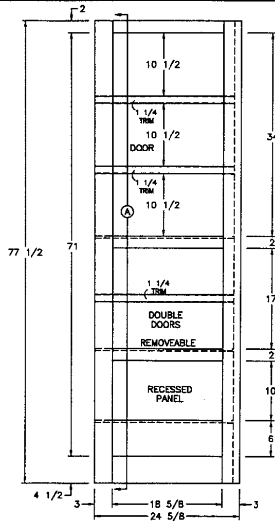
FRONT VIEW
