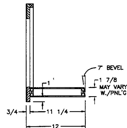
SIDE SECTION (A)
