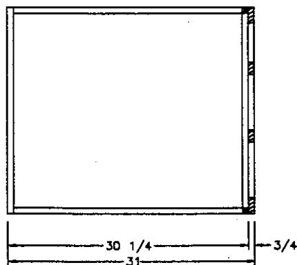
SIDE SECTION (A)
