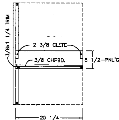
SIDE SECTION (A)
