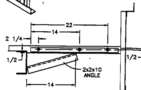
FRONT-FACING SIDE VIEW
