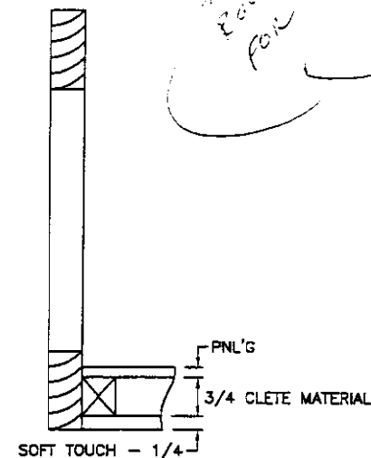
SIDE SECTION (A) ENLARGED 5X
