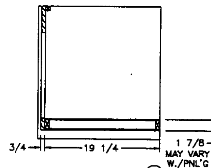
SIDE SECTION (B)
