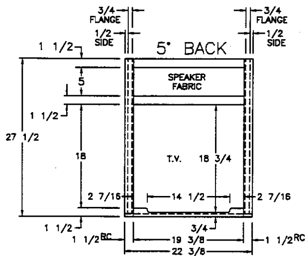
FRONT VIEW (FRONT)
