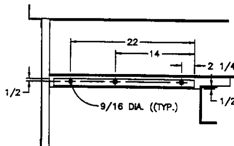
REAR-FACING SIDE VIEW
