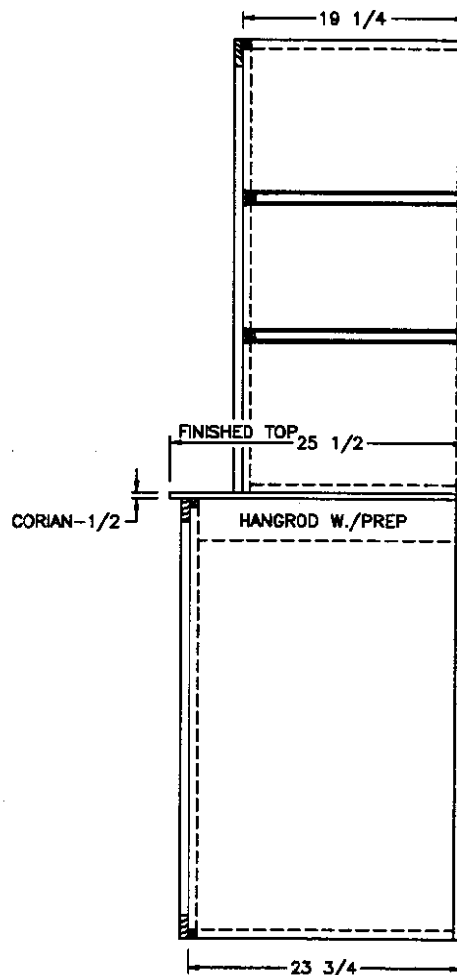
SIDE SECTION (A)
