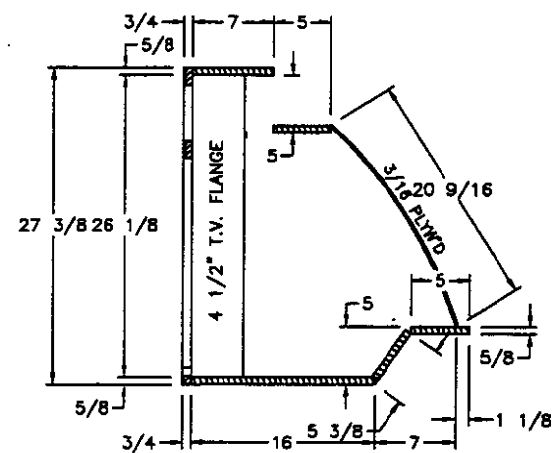
SIDE SECTION (A)
