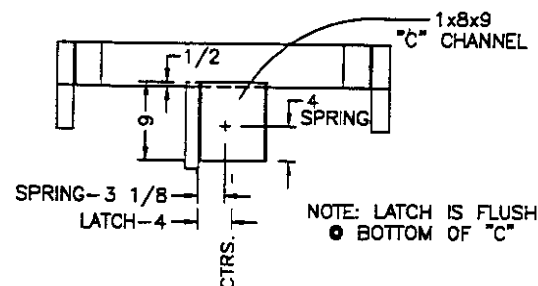
REAR END VIEW
