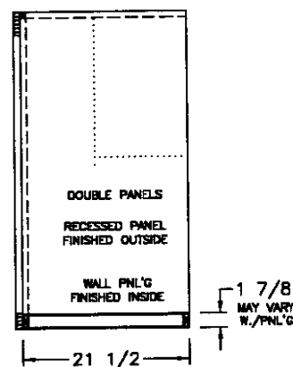
SIDE SECTION (C)
