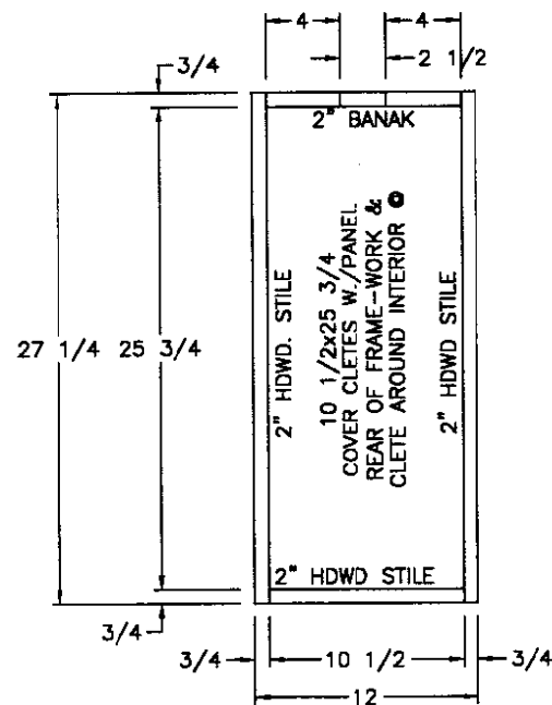
FRONT VIEW OF FRAME-WORK
