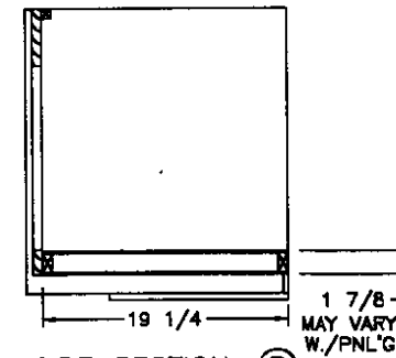
SIDE SECTION (B)
