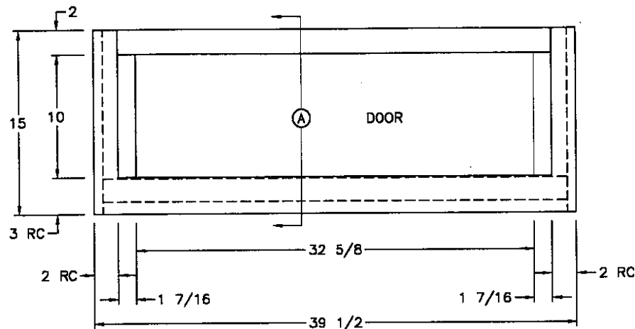
FRONT VIEW (2) 16 1/2x11 1/2 GLASS DOORS
