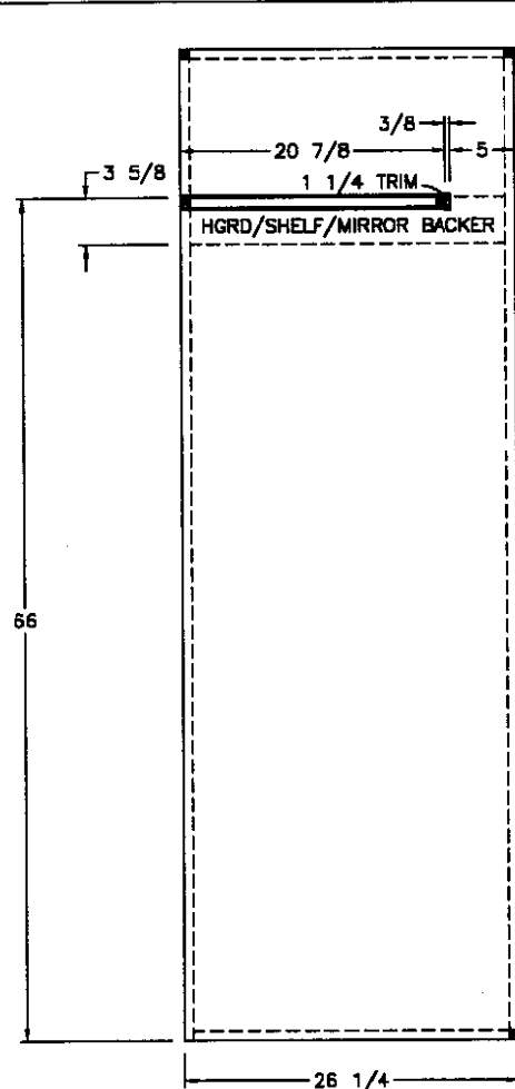
SIDE SECTION (A) (2) 12 1/2x71 1/2 MIRROR DOORS
