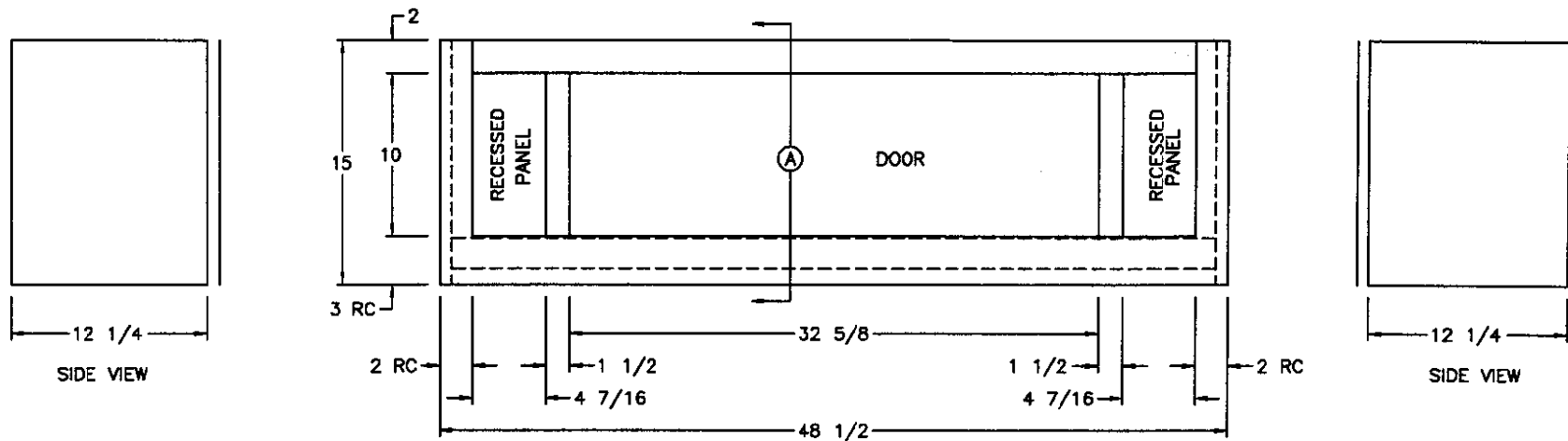
FRONT VIEW (2) 16 1/2x11 1/2 GLASS DOORS
