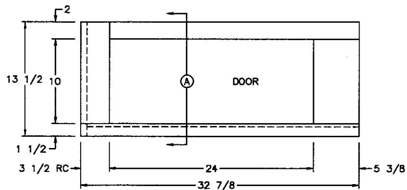
FRONT VIEW (1) 24 1/2x10 1/2 DOOR
