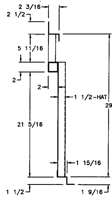
SIDE PROFILE (B)
