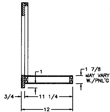
SIDE SECTION (A)
