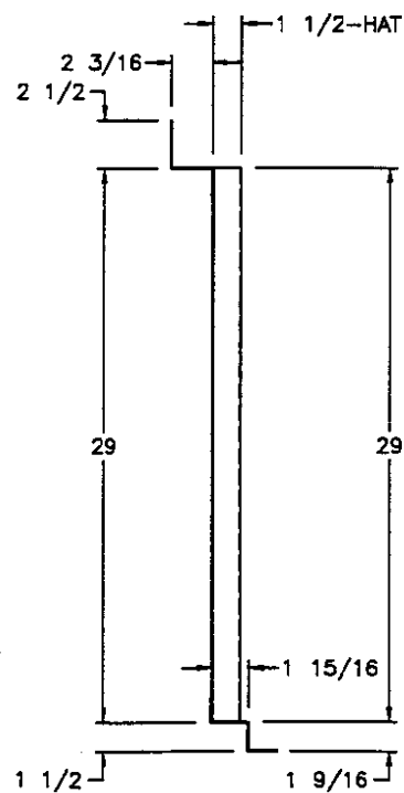
SIDE PROFILE (A)
