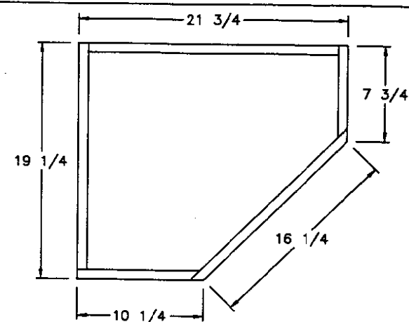
BOTTOM PANEL
