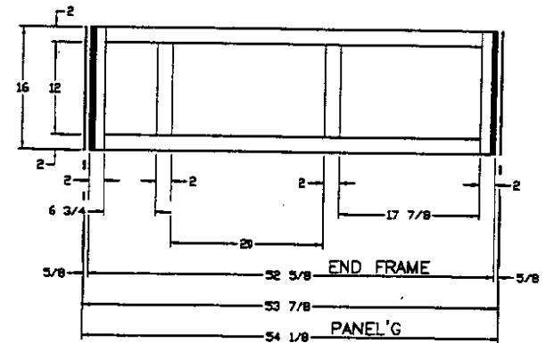
END (INTERIOR VIEW)
