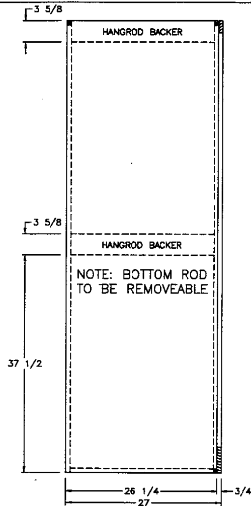
SIDE SECTION (A) (2) 12 1/2x71 1/2 MIRROR DOORS
