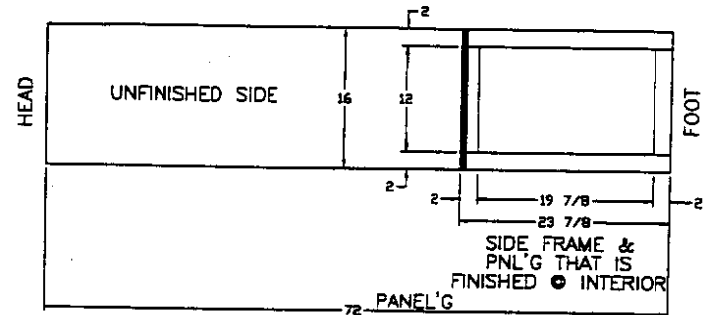
SIDE (INTERIOR VIEW) (2) SIDES REQ'D (LEFT/RIGHT)
