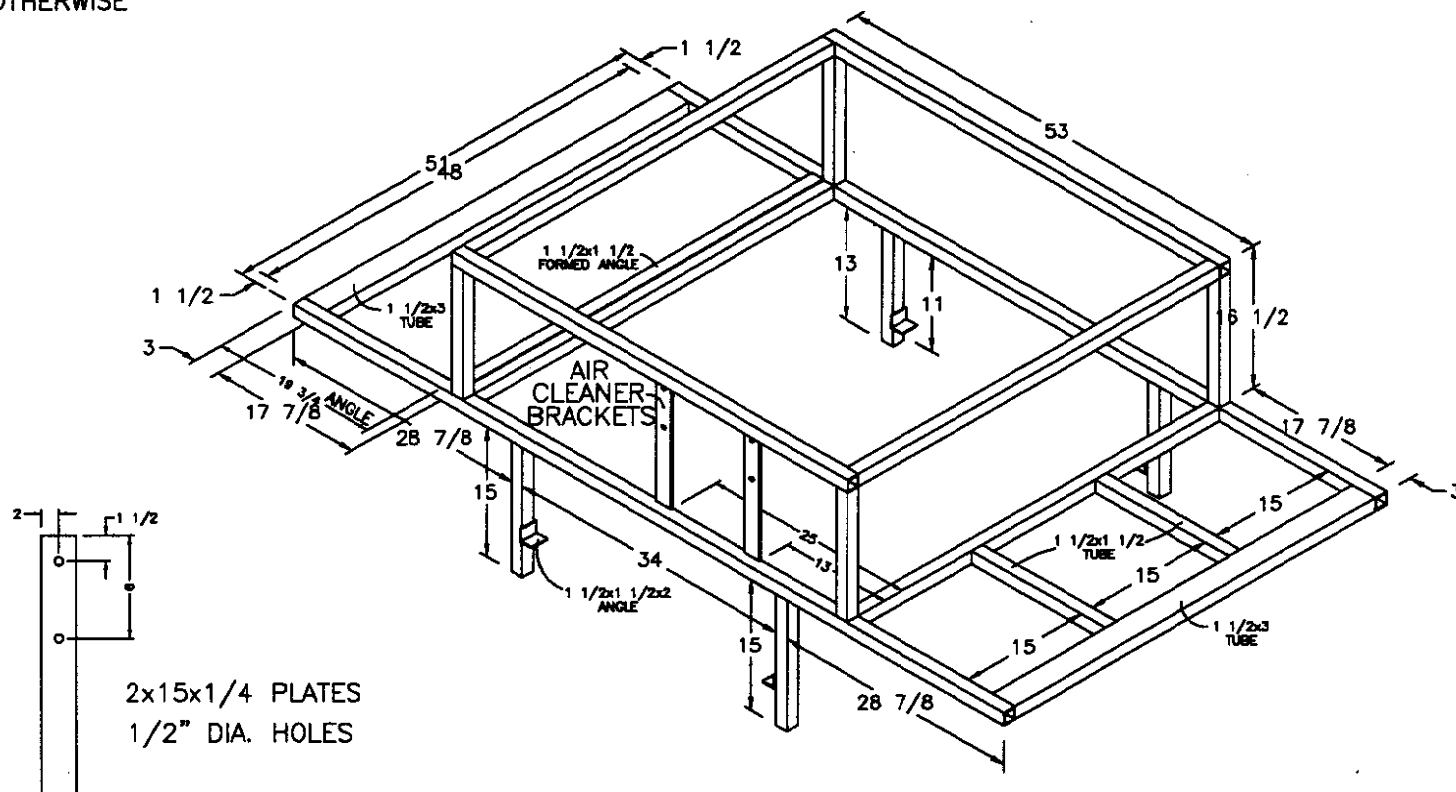
AIR CLEANER MTG. BRACKET
