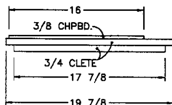
(B) VIEW (SEE TOP VIEW)
