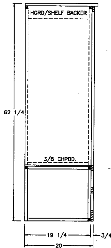
SIDE SECTION (A)
