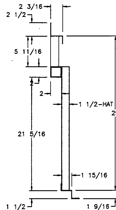
SIDE PROFILE (B)
