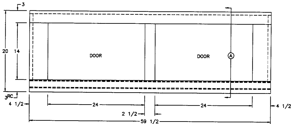
FRONT VIEW
