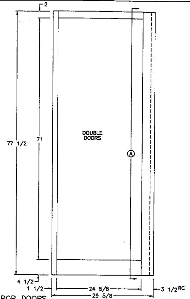
FRONT VIEW
