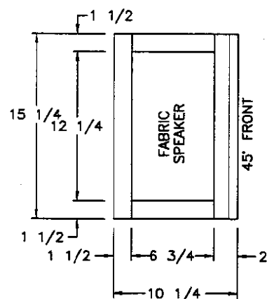
LFT END VIEW
