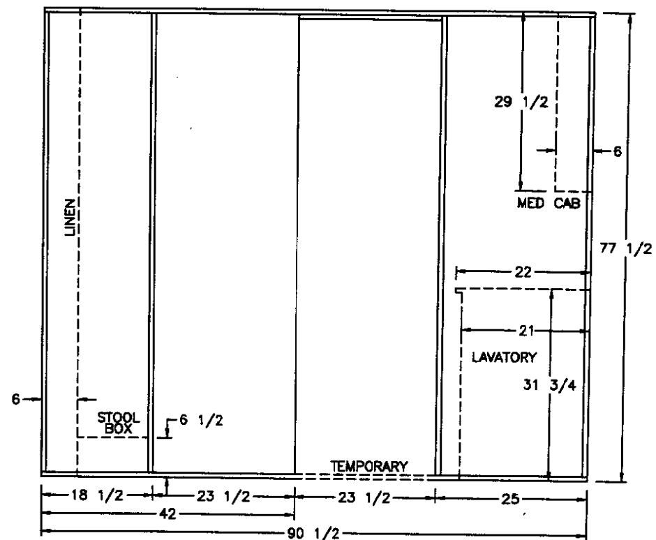
VIEW (B)
