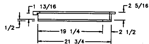
SIDE SECTION
