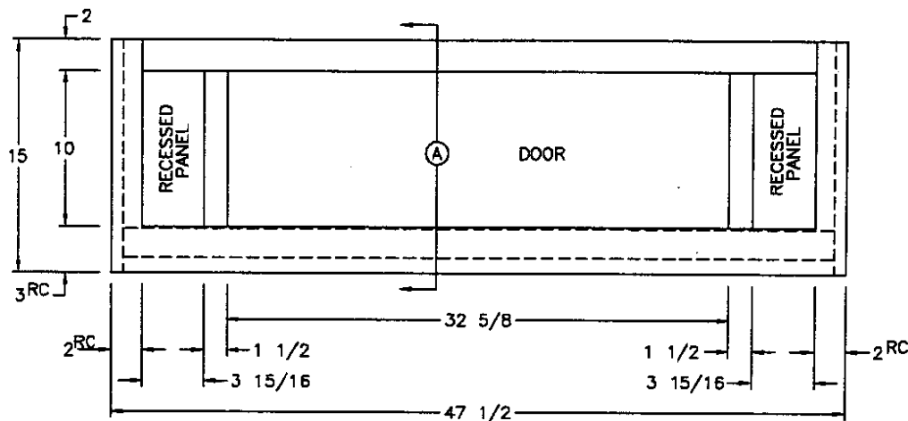
FRONT VIEW (2) 16 1/2x11 1/2 GLASS DOORS
