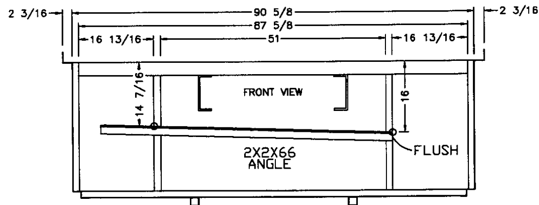
REAR HOLDING TANK CROSSMEMBER
