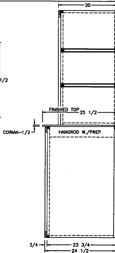
SIDE SECTION (A)
