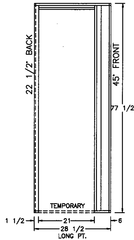
VIEW (F)
