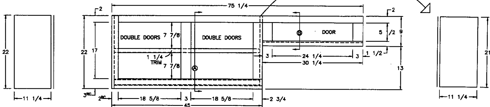
FRONT VIEW
