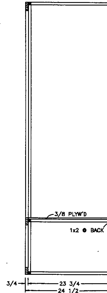
SIDE SECTION (A)
