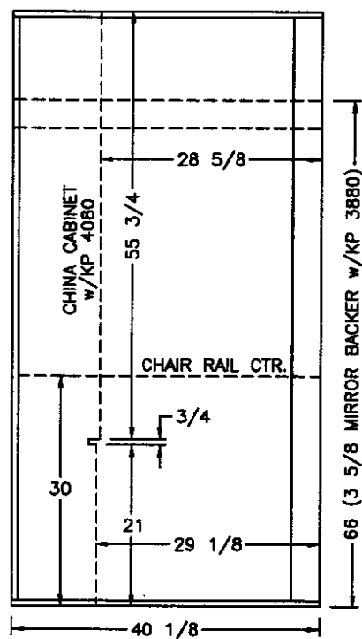
VIEW H
