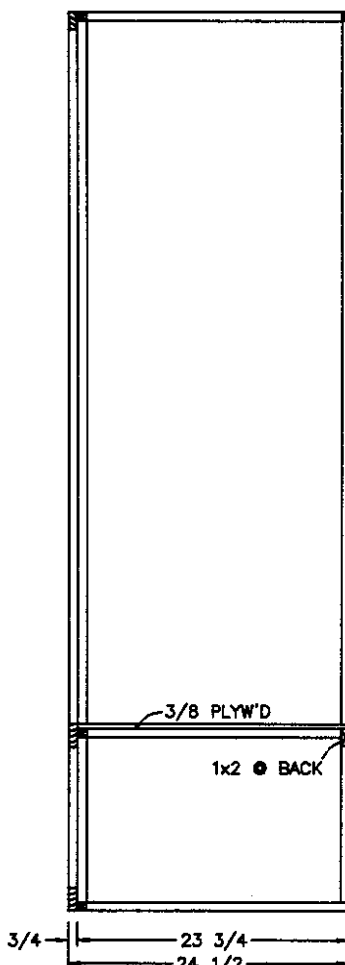
SIDE SECTION (A)
