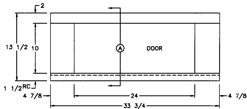
FRONT VIEW (1) 24 1/2x10 1/2 DOOR
