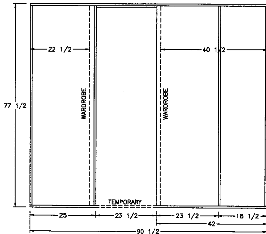
VIEW (A)
