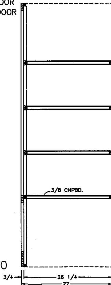
SIDE SECTION (B)
