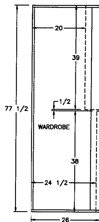
VIEW ©
