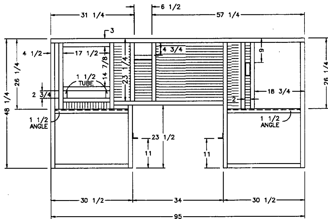
1 1/2 TUBES FRONT/EXTERIOR VIEW
