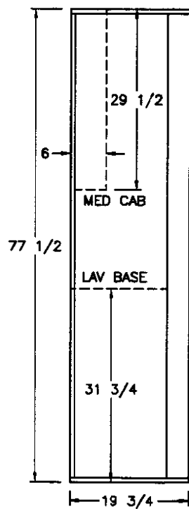
VIEW ©
