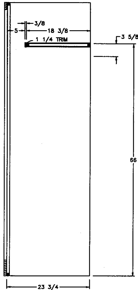
SIDE SECTION (A)
