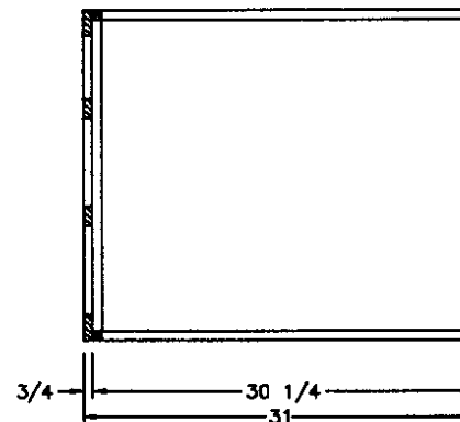
SIDE SECTION (B)
