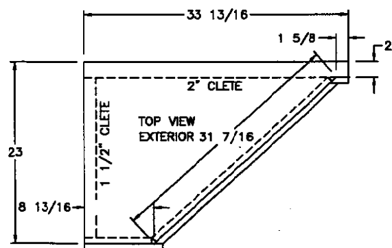
OFFDOOR SIDE
