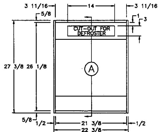
FRONT VIEW (FRAME)
