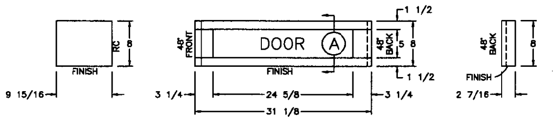
OFFDOOR SIDE FRONTS (1) 25 1/8x5 1/2 DOOR
