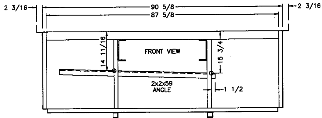
FRONT HOLDING TANK CROSSMEMBER
