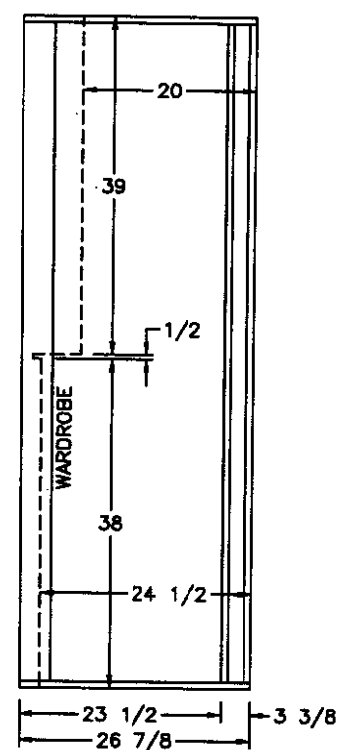
VIEW I
