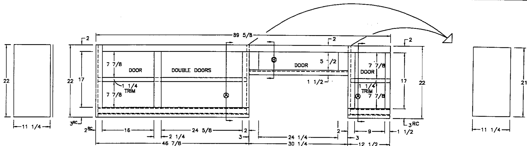
FRONT VIEW
