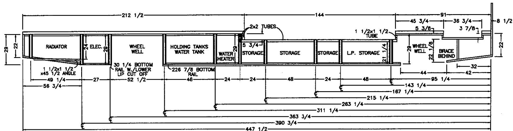
OFFDOOR SIDE
