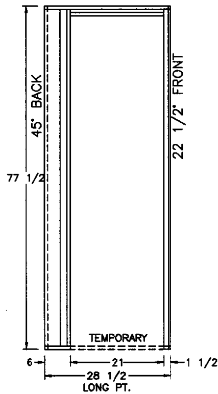
VIEW (E)
