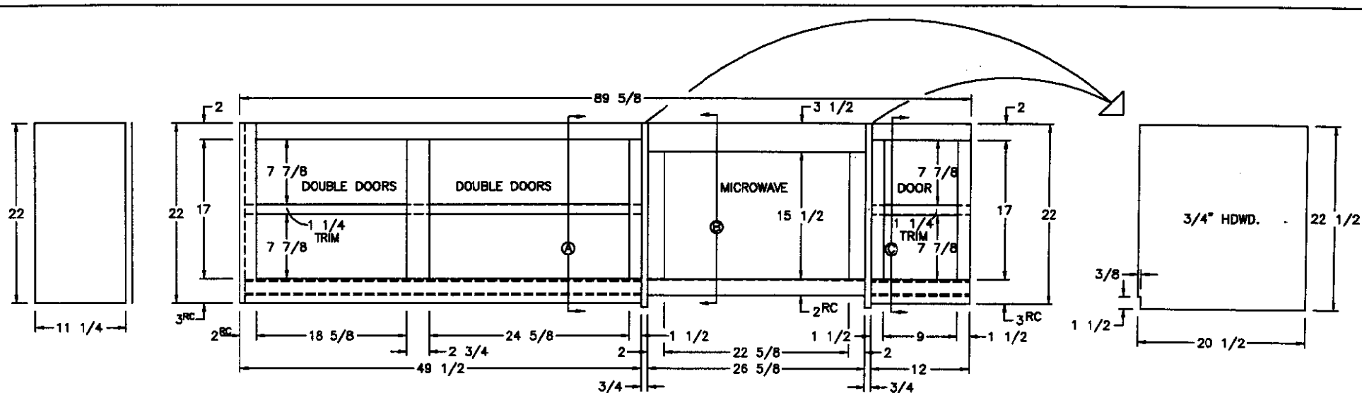
FRONT VIEW (3) 9 1/2x18 1/2 DOORS (2) 12 1/2x18 1/2 DOORS
