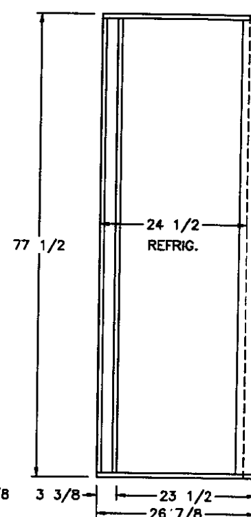
VIEW J
