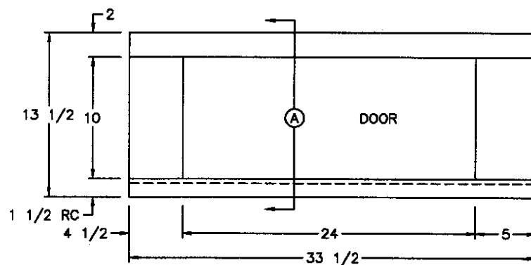
FRONT VIEW (1) 24 1/2x10 1/2 DOOR
