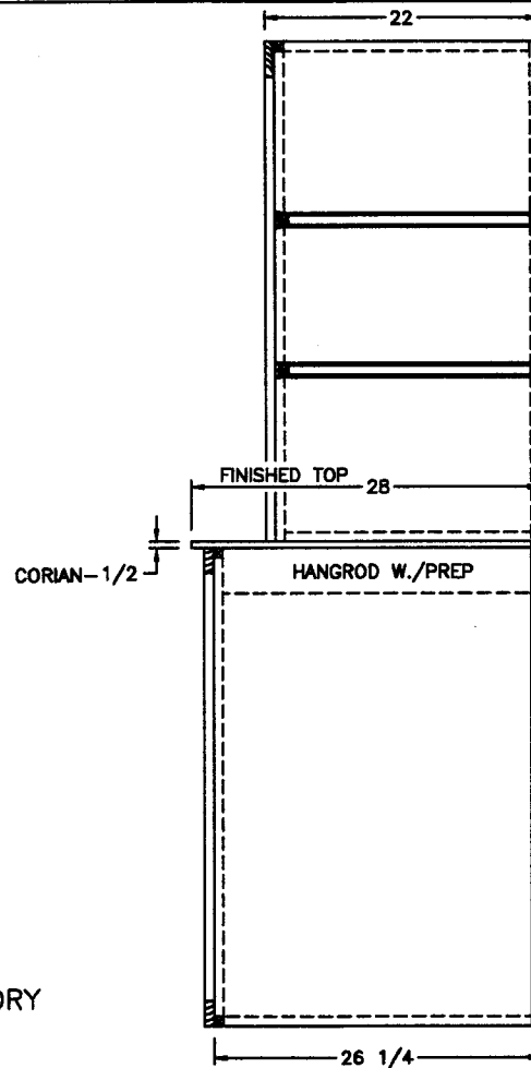
SIDE SECTION (A)
