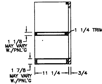
SIDE SECTION (C)
