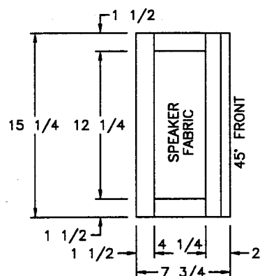
LFT END VIEW
