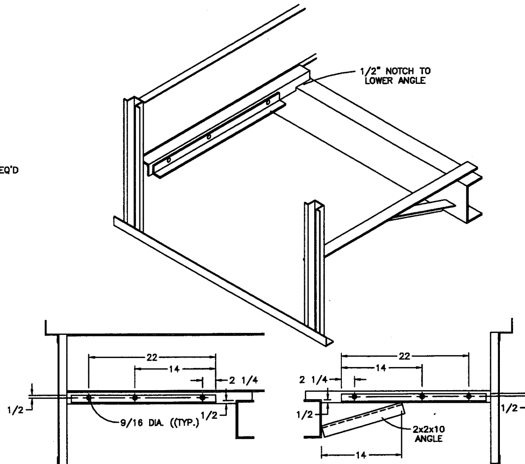
REAR-FACING SIDE VIEW
