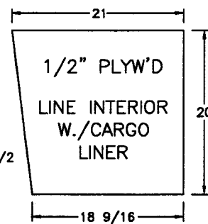
DETAIL B - SIDES (2) REQ'D
