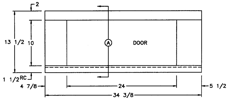
FRONT VIEW (1) 24 1/2x10 1/2 DOOR
