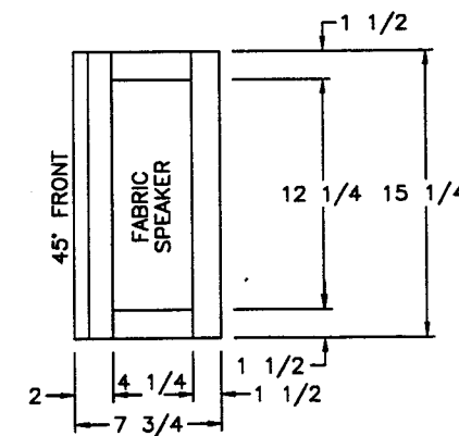
RT END VIEW
