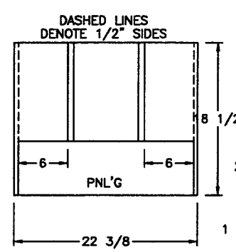
DETAIL C - BOTTOM 1/2" PLYW'D
