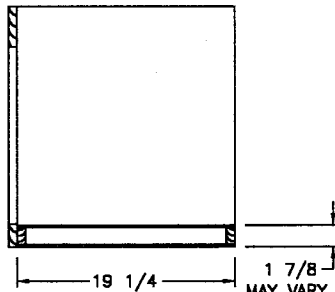
SIDE SECTION (B)
