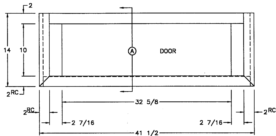
FRONT VIEW (2) 16 1/2x10 1/2 DOORS
