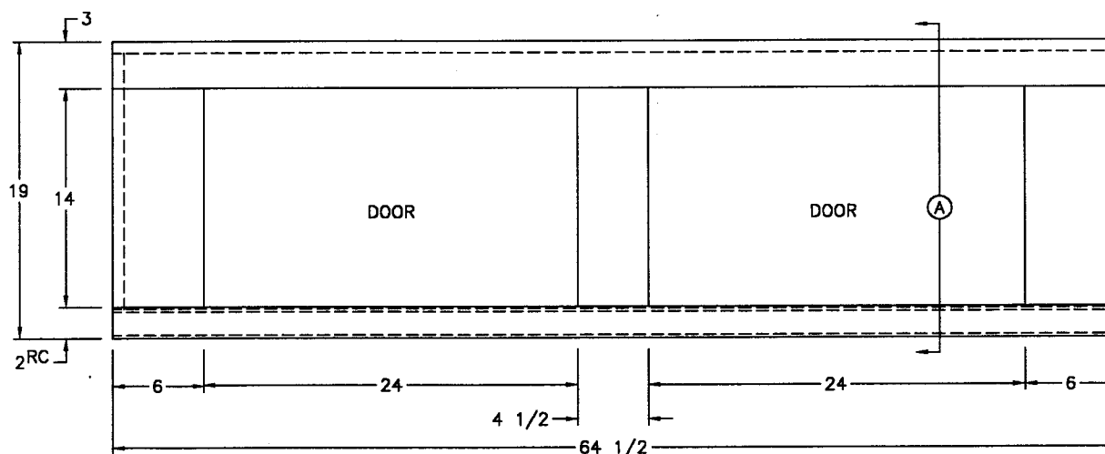
(2) 24 1/2x14 1/2 DOORS
