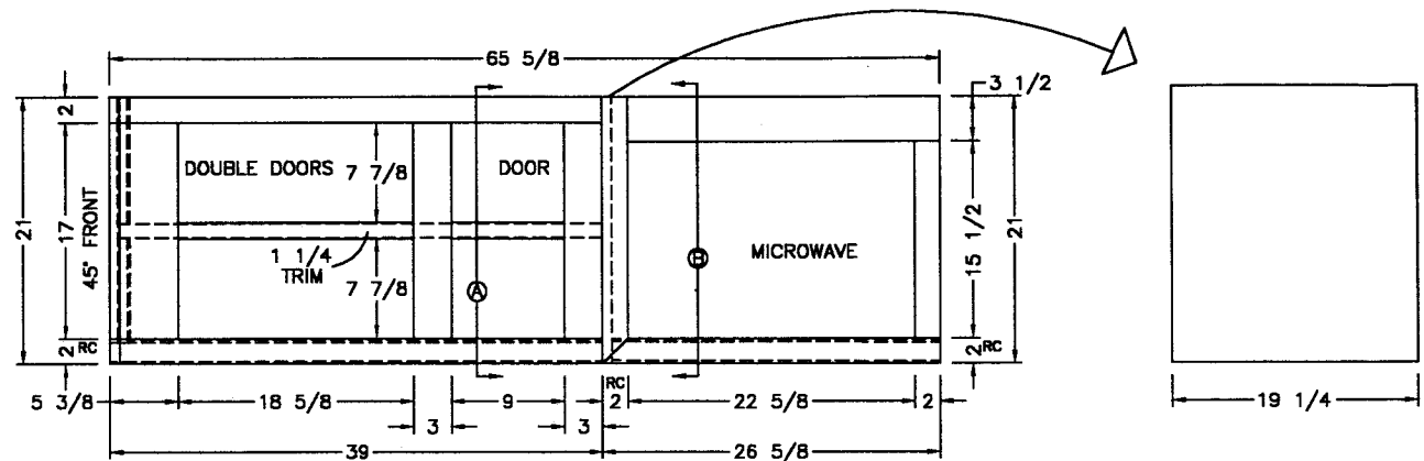
FRONT VIEW
