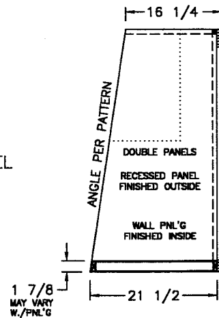
SIDE SECTION ©
