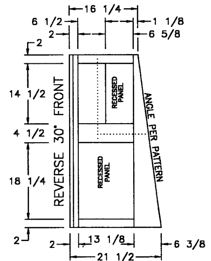
END PANEL
