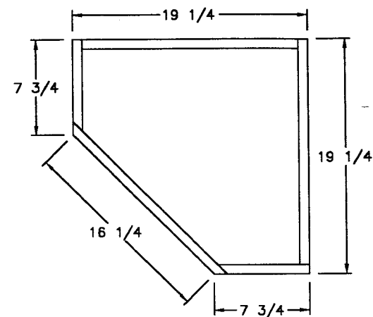
BOTTOM PANEL
