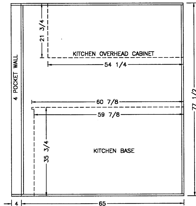
VIEW (F)
