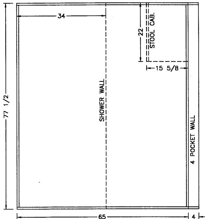
VIEW (E)
