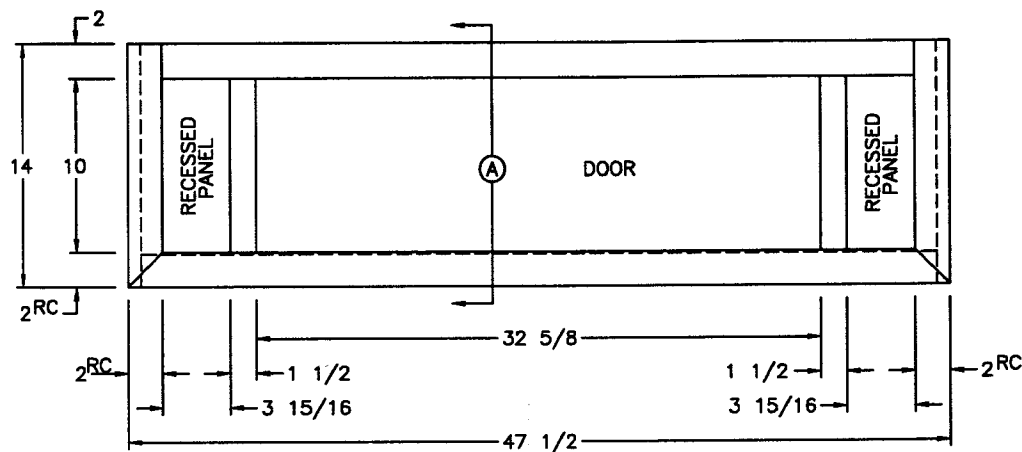
FRONT VIEW (2) 16 1/2x10 1/2 DOORS
