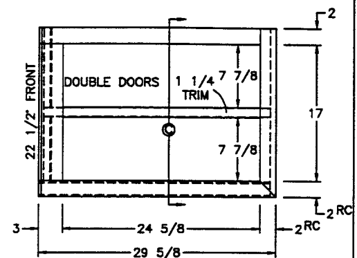
(2) 12 1/2x17 1/2 DOORS
