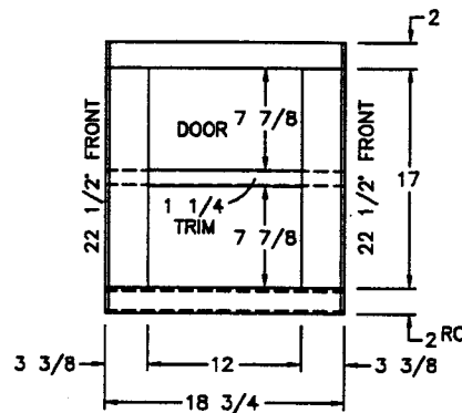
(1) 12 1/2x17 1/2 DOORS
