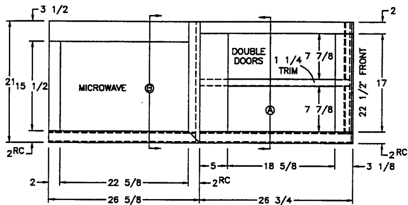
(2) 9 1/2x17 1/2 DOORS
