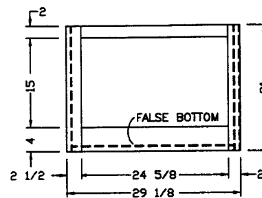
CHINA HUTCH BASE FRONT VIEW
