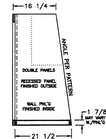
SIDE SECTION ©
