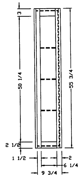
CHINA HUTCH OVERHEAD SIDE VIEW
