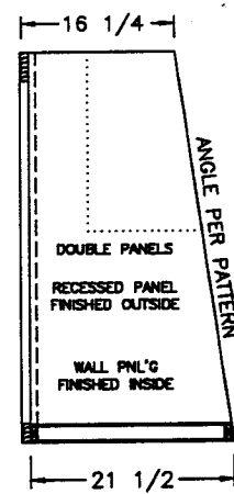
SIDE SECTION ©
