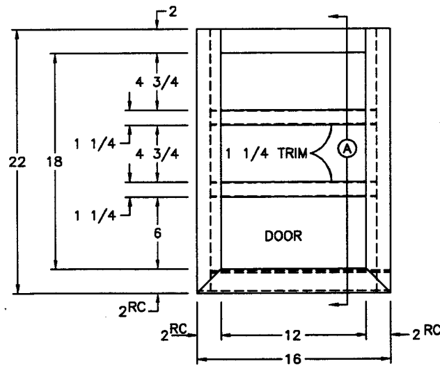
FRONT VIEW (1) 12 1/2x18 1/2 DOOR
