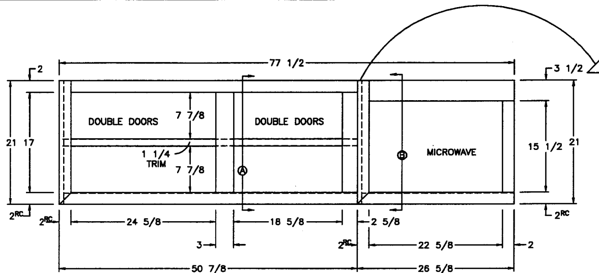
FRONT VIEW
