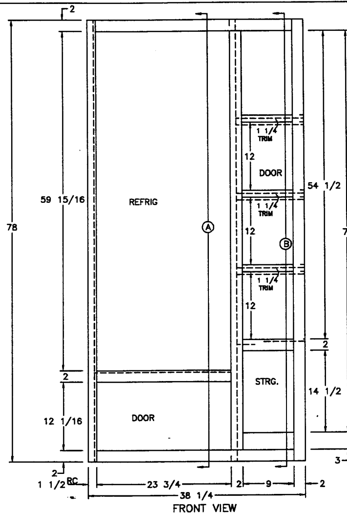
FRONT VIEW
