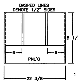
DETAIL C - BOTTOM 1/2" PLYW'D
