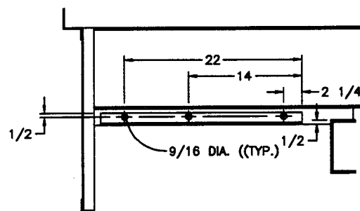
REAR-FACING SIDE VIEW
