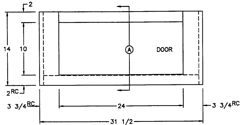
FRONT VIEW (1) 24 1/2x10 1/2 GLASS DOOR
