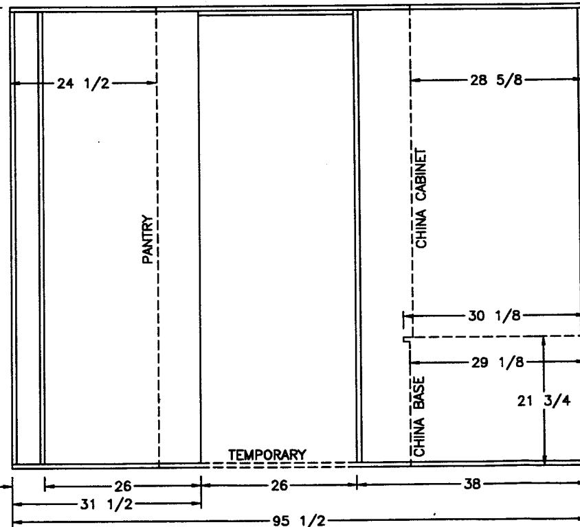
VIEW D
