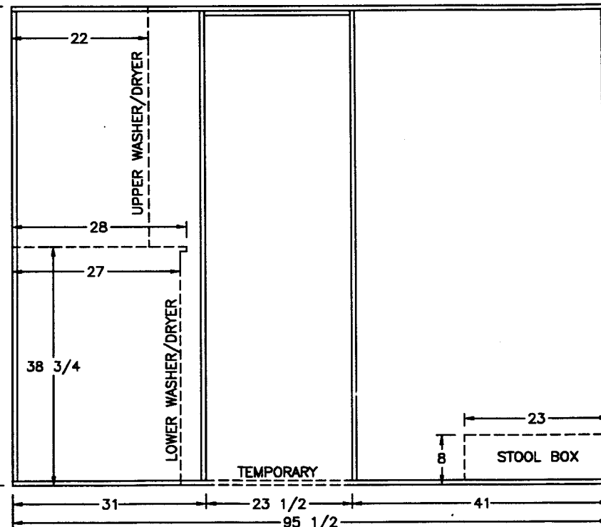
VIEW (B)
