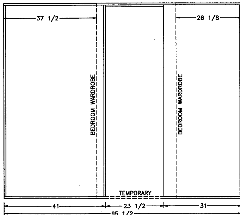
VIEW (A)
