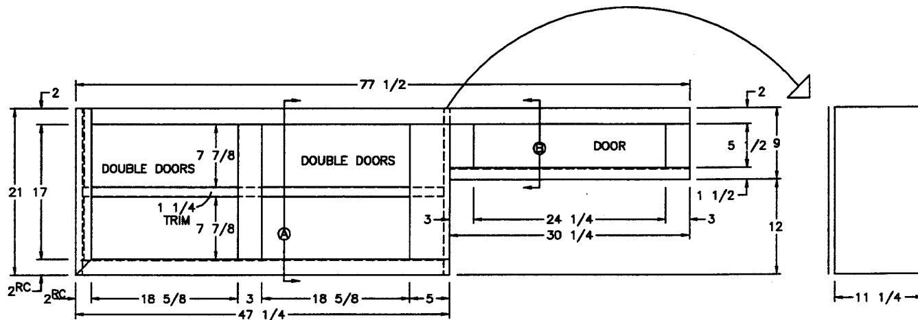
FRONT VIEW
