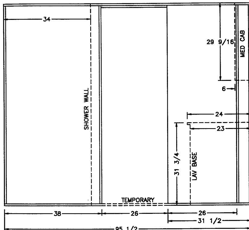
VIEW C
