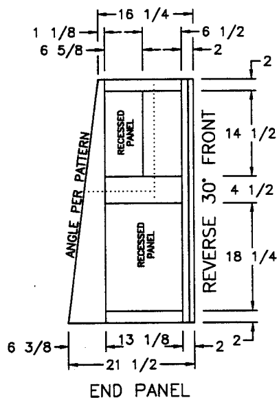
END PANEL
