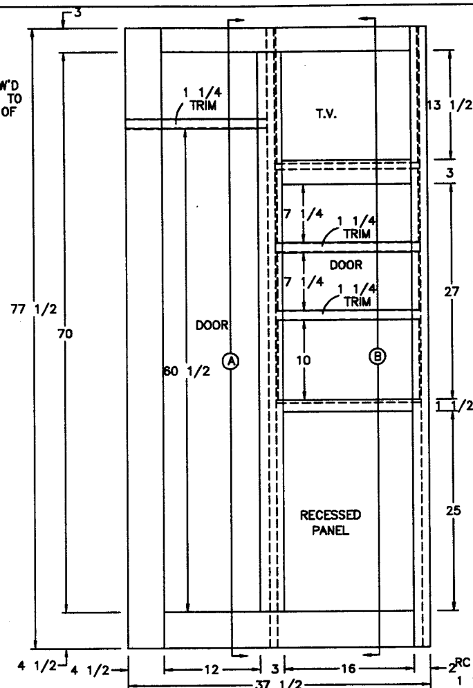
FRONT VIEW (1) 12 1/2x71 1/2 MIRROR DOOR (1) 16 1/2x27 1/2 DOOR
