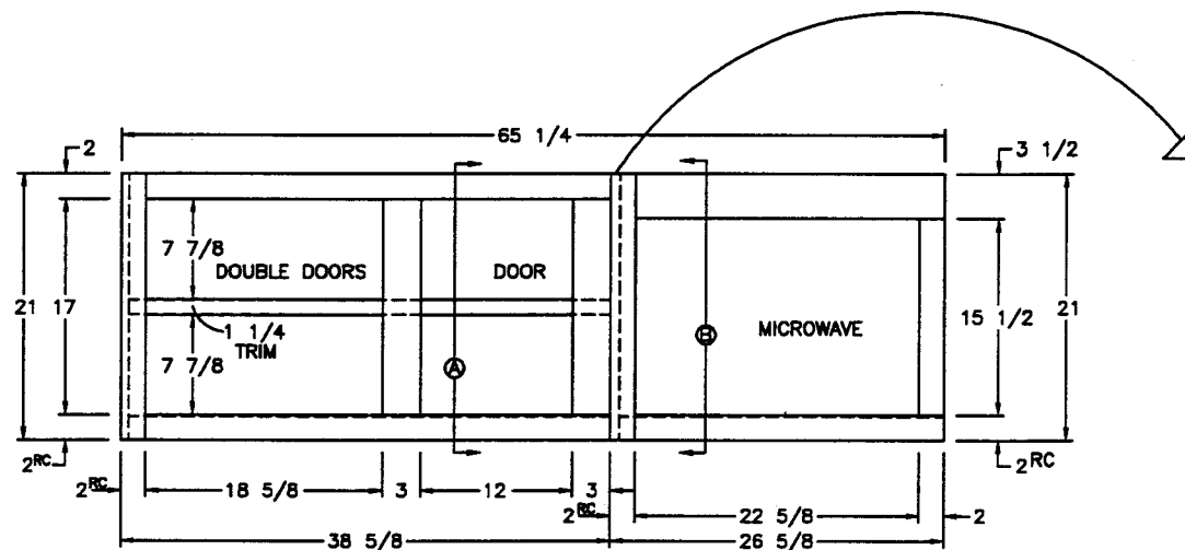
FRONT VIEW (2) 9 1/2x17 1/2 DOORS (1) 12 1/2x17 1/2 DOORS
