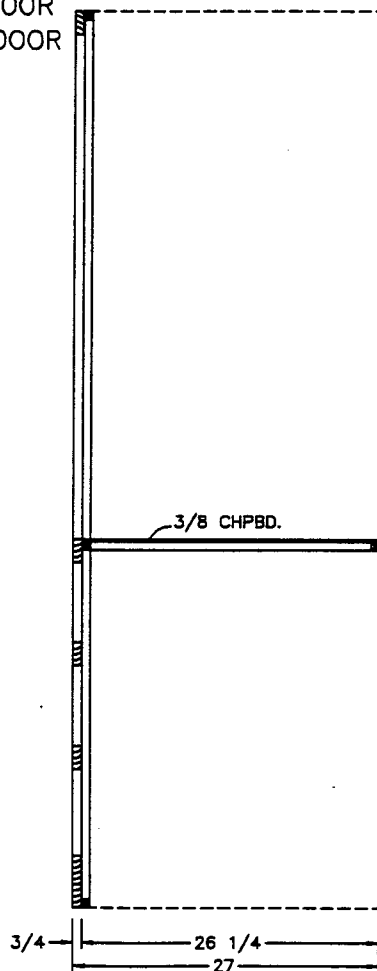
SIDE SECTION (B)
