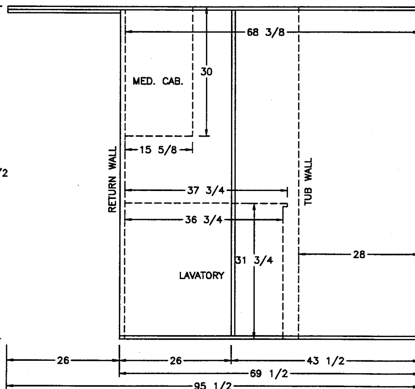
VIEW (B)
