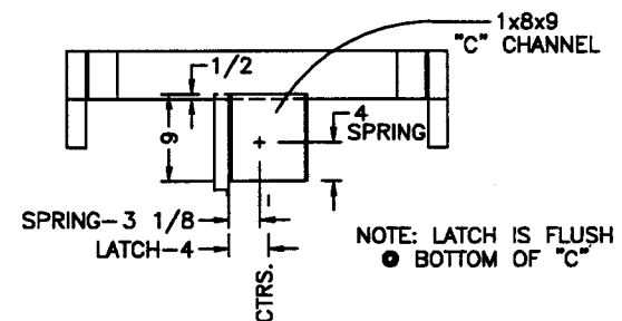
REAR END VIEW
