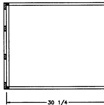
SIDE SECTION (B)
