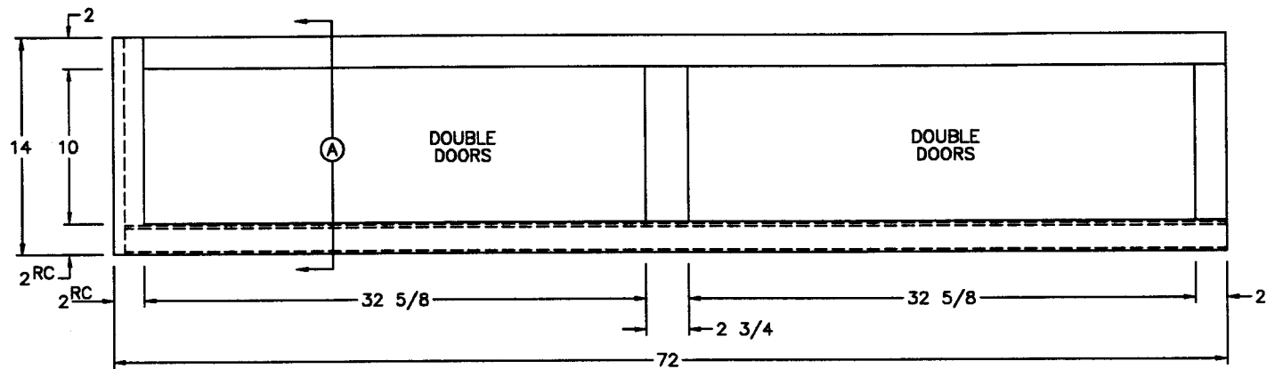
FRONT VIEW (4) 16 1/2x11 1/2 DOORS
