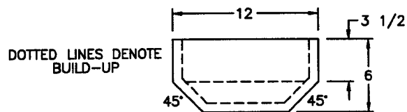
TOP VIEW OF FRAME TOP
