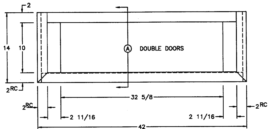
FRONT VIEW (2) 16 1/2x10 1/2 DOORS
