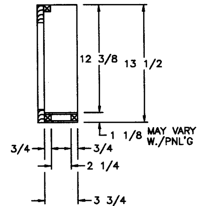
SIDE SECTION (A)
