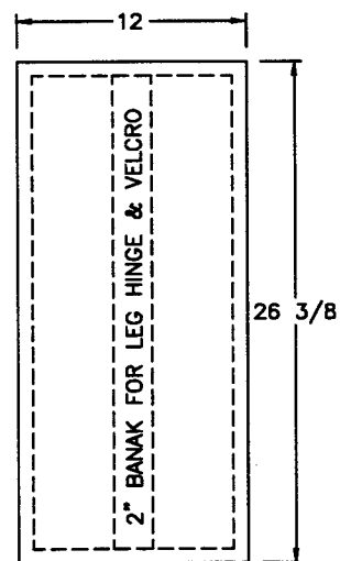
DOTTED LINES DENOTE BUILD-UP TOP VIEW OF TABLE
