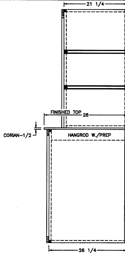
SIDE SECTION (A)
