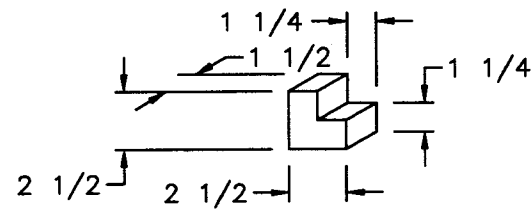
WALL BLOCK FOR WATER LINES TWO PER UNIT REQ'D
