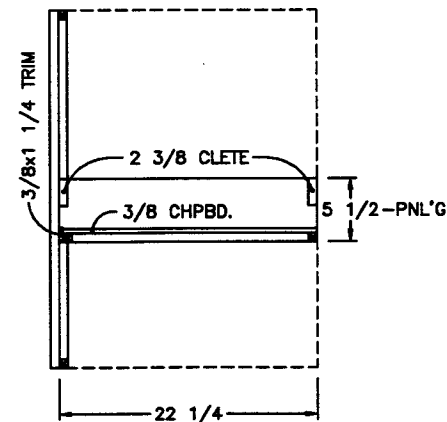
SIDE SECTION (A)
