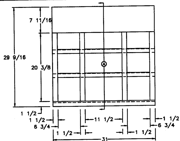
FRAME-WORK DECORATIVE WALL PANEL TOP BETWEEN MIRROR FRAME & CEILING
