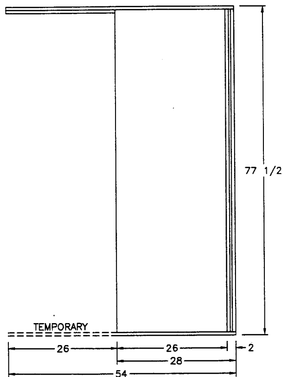
VIEW (A)
