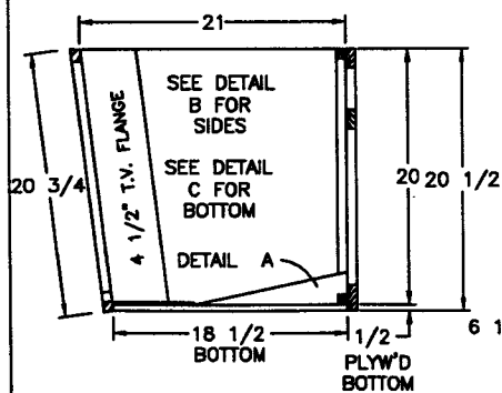
SIDE SECTION (A)
