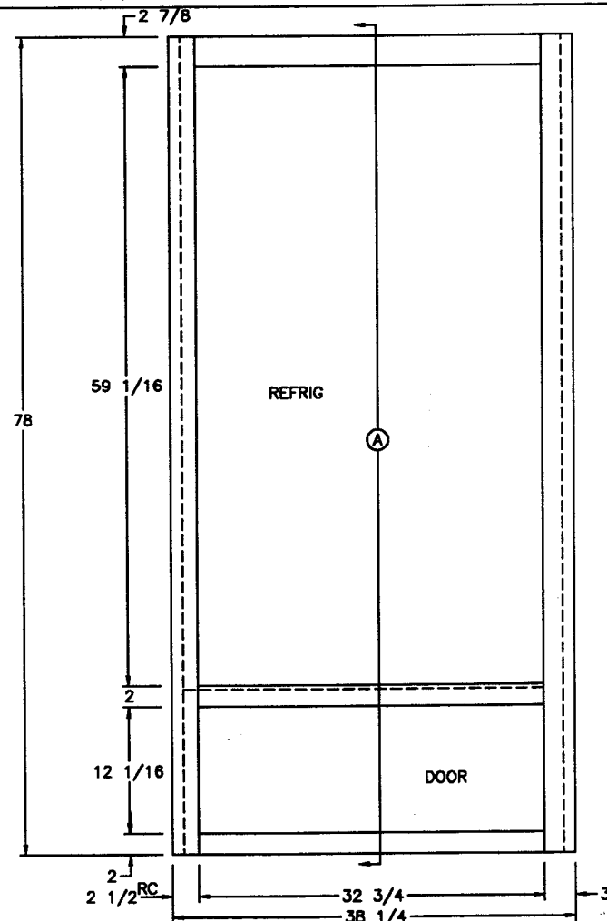
FRONT VIEW
