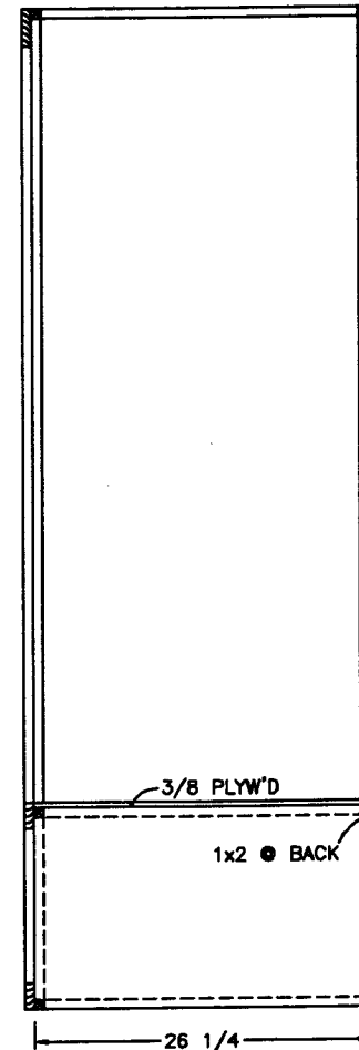
SIDE SECTION (A)
