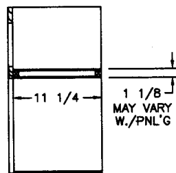
SIDE SECTION (B)
