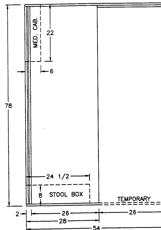
VIEW (B)
