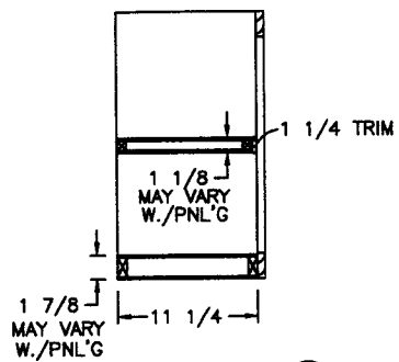
SIDE SECTION (A)
