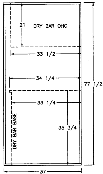
VIEW (F)
