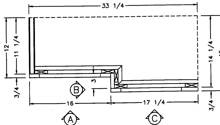
BASE
