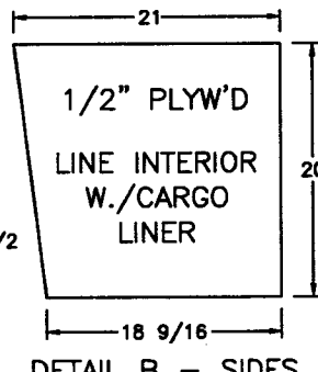
DETAIL B - SIDES (2) REQ'D
