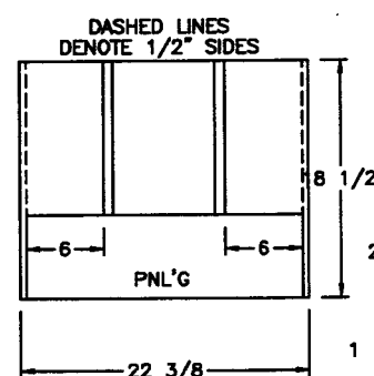
DETAIL C - BOTTOM 1/2" PLYW'D
