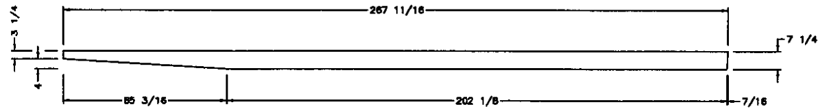
Wood header detail
