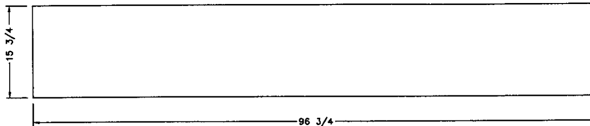
FRONT SUPER STORAGE RISER RISER MADE UP WITH 5/8" PLYWOOD AND METAL ON THE FRONT SIDE
