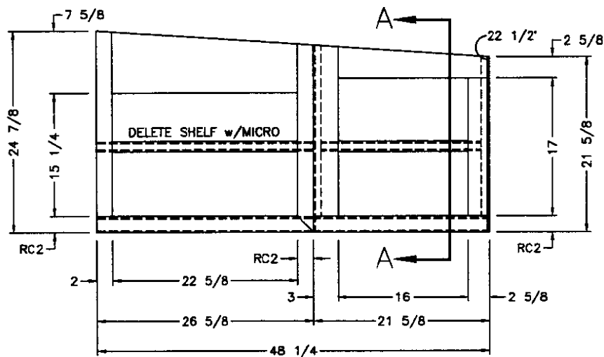
SIDE OVERHEAD (FRONT VIEW) 20" DEPTH 12" DEPTH
