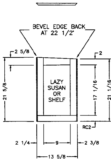
CORNER OVERHEAD (1) 9 1/2 X 17 1/2
