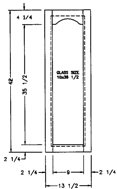
FRONT GLASS HINGED DOOR
