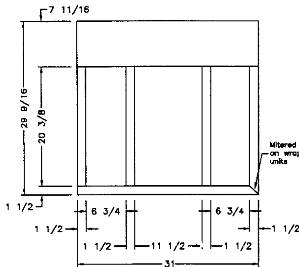
STILE FRAMING 3/4" THICK PANEL
