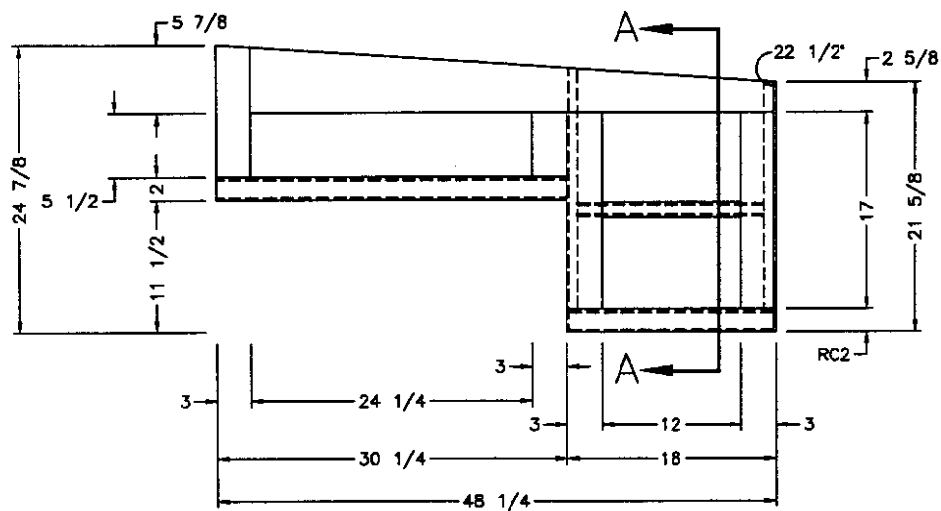
SIDE OVERHEAD (FRONT VIEW) 12" DEPTH
