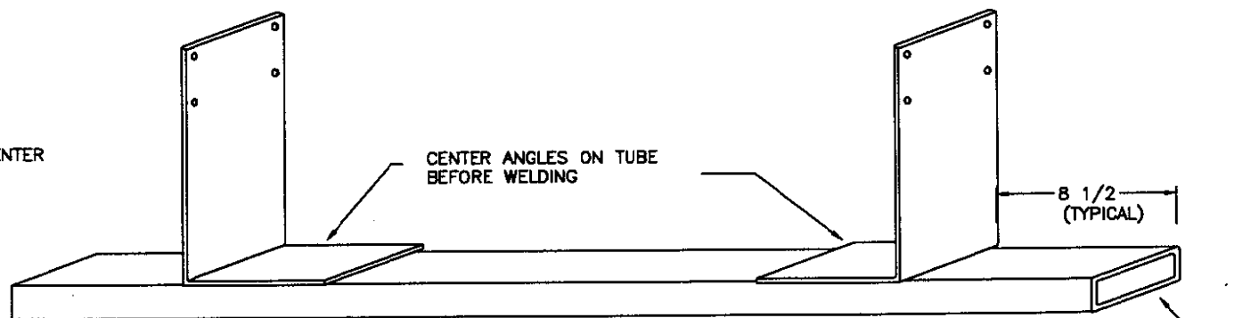
ASSEMBLED ISO VIEW
