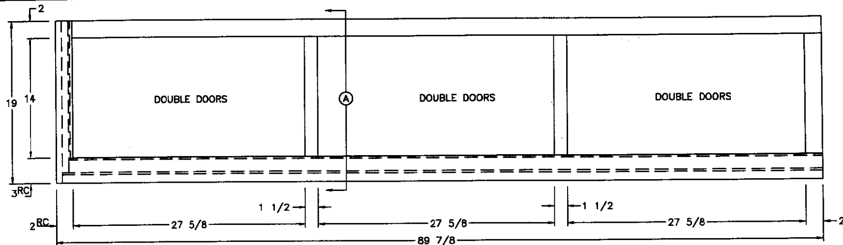
FRONT VIEW (6) 14x15 1/2 DOORS
