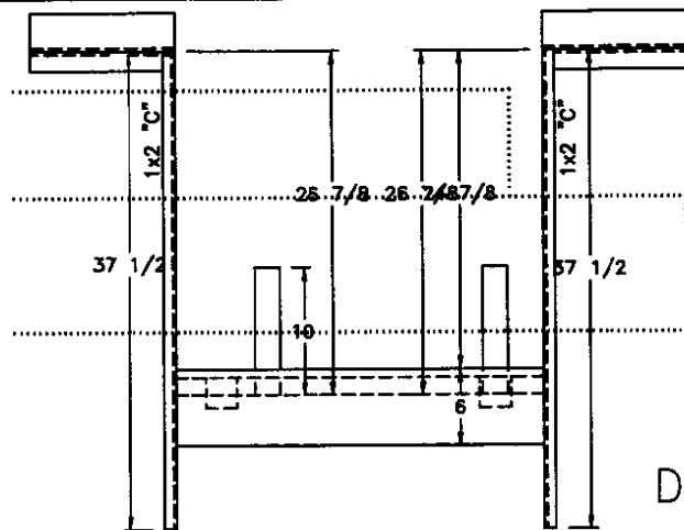
FRONT VIEW (DOOR SIDE)
