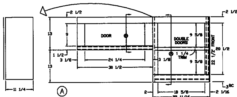
(1) 24 3/4x10 DOOR (2) 9 1/2x22 1/2 GLASS DOORS
