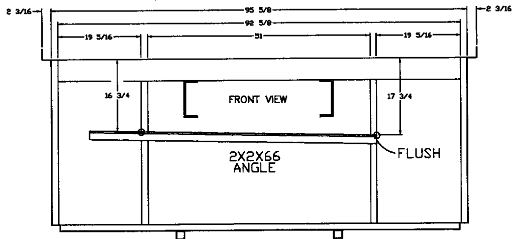
REAR HOLDING TANK CROSSMEMBER
