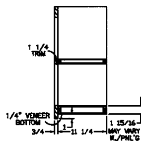
SIDE SECTION (A)
