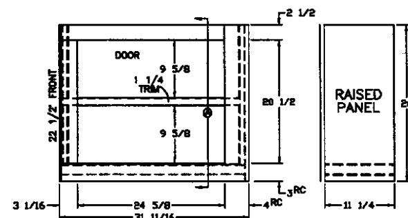
(2) 12 1/2x22 1/2 GLASS DOORS
