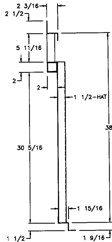
SIDE PROFILE (B)
