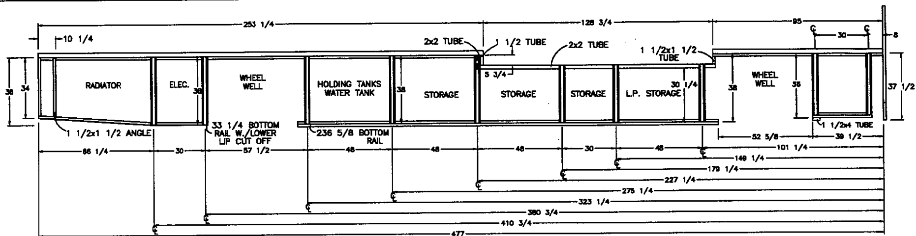
OFFDOOR SIDE
