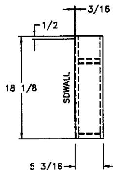
BACK END
