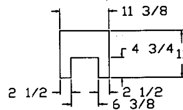
Plywood detail
