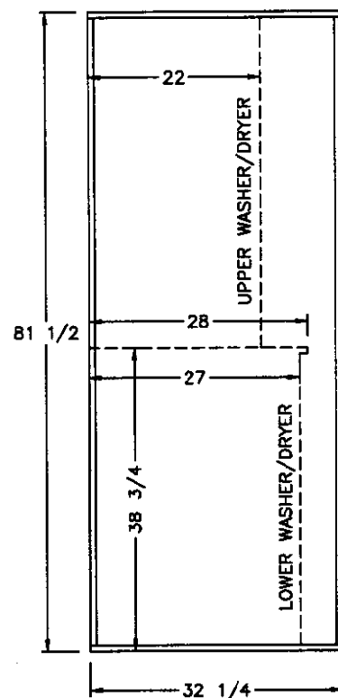
VIEW (C)
