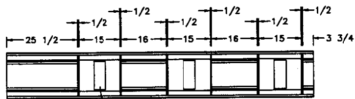
4 1/8x10 CENTERED (TYP) View from top looking down
