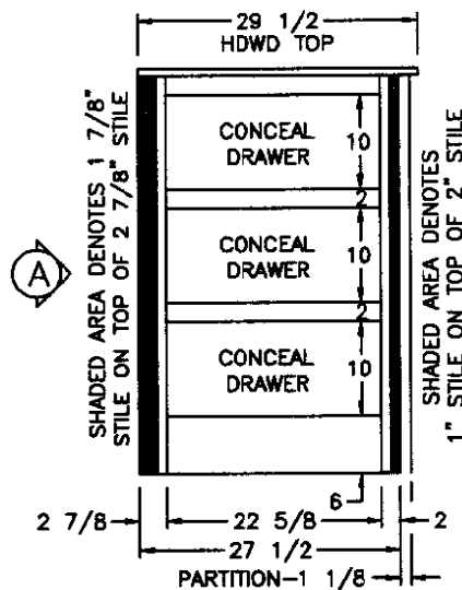
INTERIOR DRAWER SECTION
