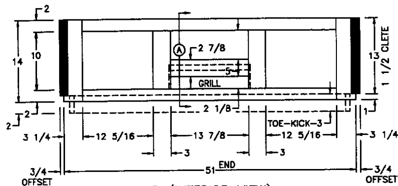
END (INTERIOR VIEW)
