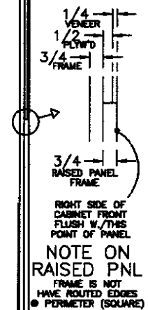
SIDE SECTION (B)
