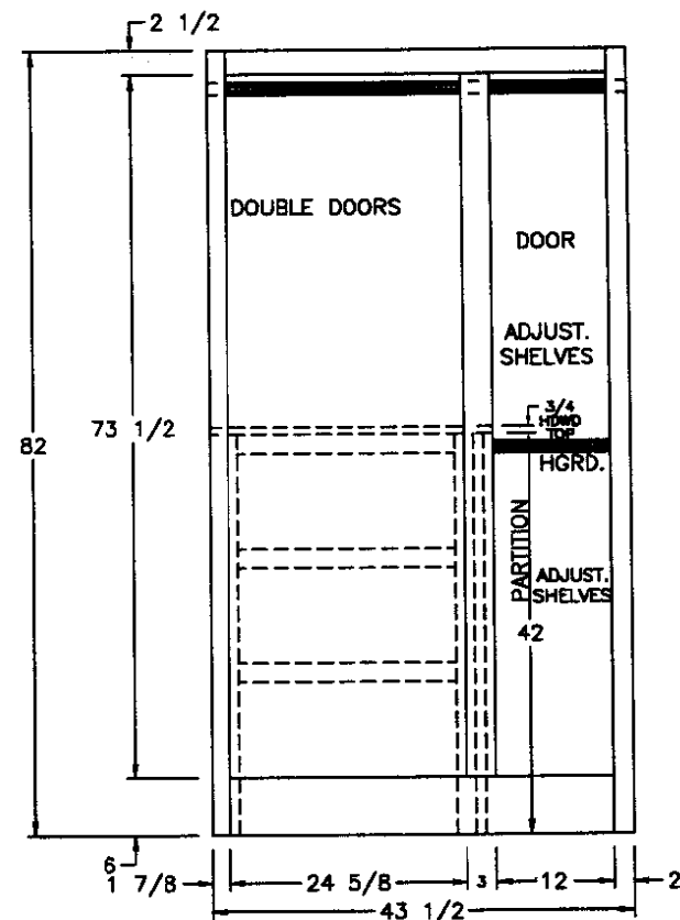
FRONT VIEW (3) 12 1/2x74 MIRROR DOORS 20" DEEP
