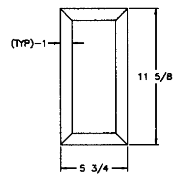
REGISTER COVER
