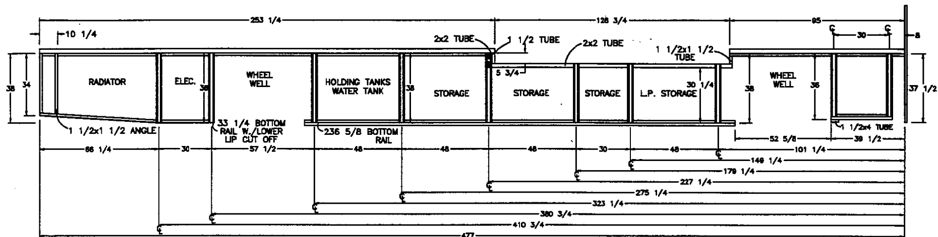
OFFDOOR SIDE
