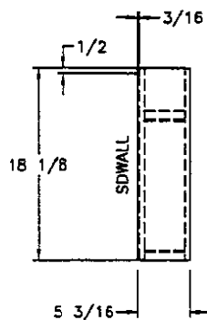
BACK END
