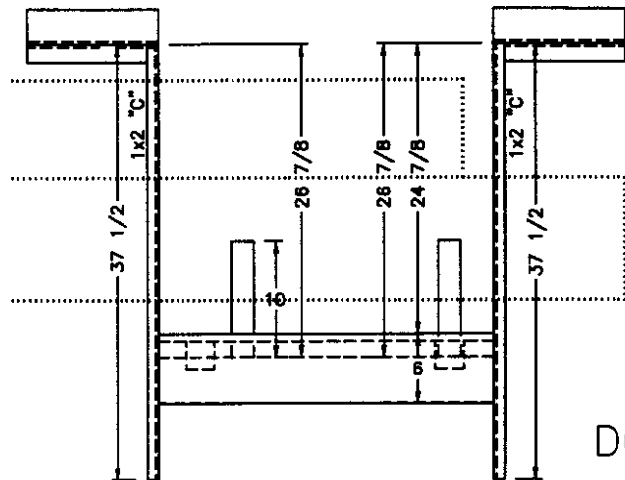
FRONT VIEW (DOOR SIDE)
