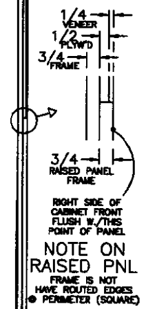
SIDE SECTION (B)
