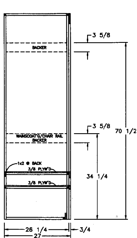
SIDE SECTION (A)
