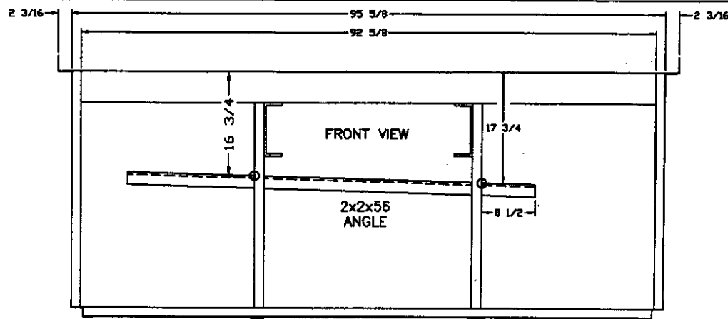
FRONT HOLDING TANK CROSSMEMBER
