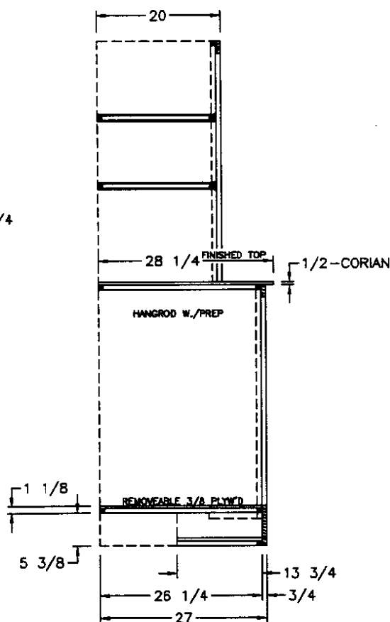
SIDE SECTION A
