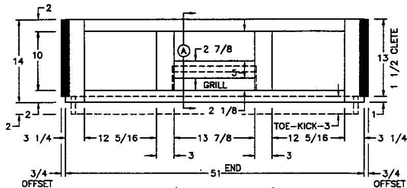
END (INTERIOR VIEW)
