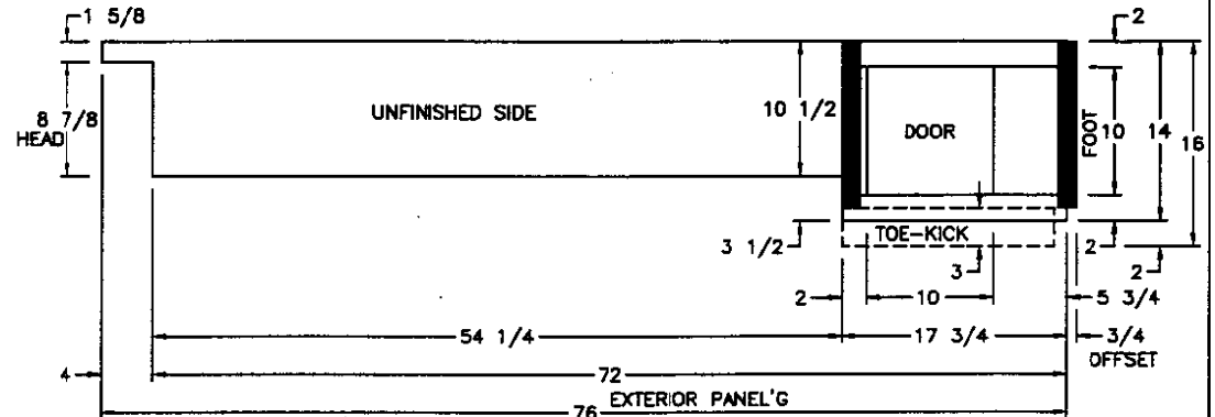
OFFDOOR SIDE (INTERIOR VIEW)
