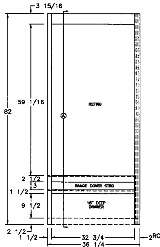
FRONT VIEW (1) 33 1/2x14 1/2 FRONT
